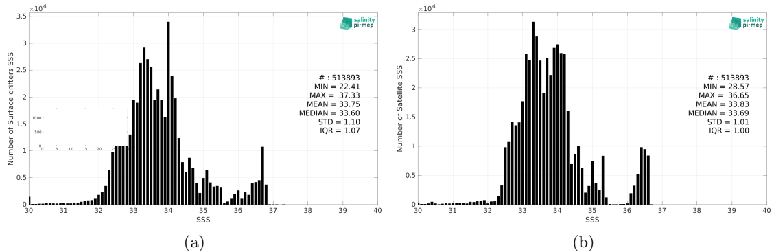
Figure 2: Histograms of SSS from Surface drifters (a) and SMAP SSS L4 OI v2 - Monthly (IPRC) (b) considering all match-up pairs per bins of 0.1 over the Tropical Pacific Ocean Pi-MEP region and for the full satellite product period.
