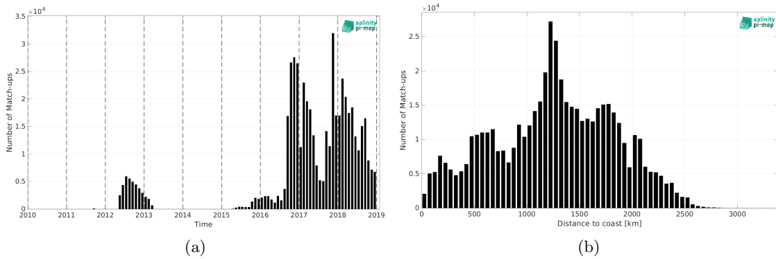
Figure 1: Number of match-ups between Surface drifters and SMAP SSS L4 OI v2 - Monthly (IPRC) SSS as a function of time (a) and as function of the distance to coast (b) over the Tropical Pacific Ocean Pi-MEP region and for the full satellite product period.
