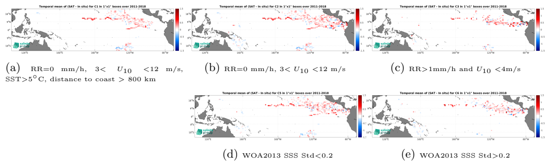
Figure 11: Temporal mean gridded over spatial boxes of size 1^\circ \times 1^\circ of \Delta SSS (SMAP SSS L4 OI v2 - Monthly (IPRC) - Surface drifters) for 5 different subdatasets corresponding to: RR=0 mm/h, 3 < U_{10} < 12 m/s, SST > 5^\circ C , distance to coast > 800 km (a), RR=0 mm/h, 3 < U_{10} < 12 m/s (b), RR > 1 mm/h and U_{10} < 4 m/s (c), WOA2013 SSS Std < 0.2 (d), WOA2013 SSS Std > 0.2 (e).
