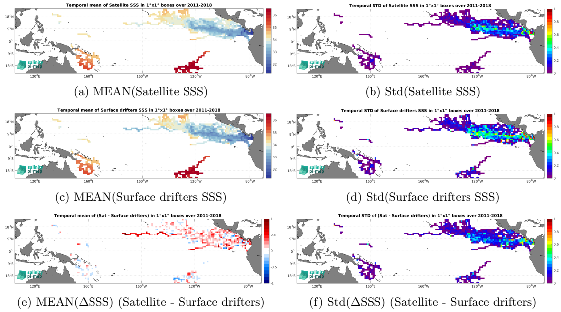
Figure 5: Temporal mean (left) and Std (right) of SSS from SMAP SSS L4 OI v2 - Monthly (IPRC) (top), Surface drifters (middle), and of \Delta SSS (Satellite - Surface drifters). Only match-up pairs are used to generate these maps.
