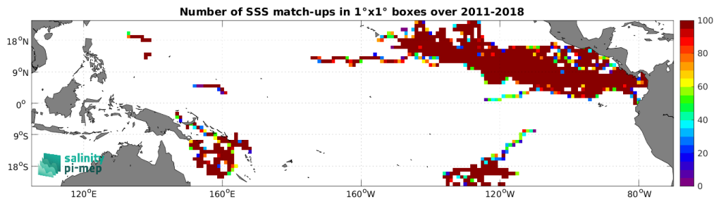
Figure 3: Number of SSS match-ups between Surface drifters SSS and the SMAP SSS L4 OI v2 - Monthly (IPRC) SSS product for the Tropical Pacific Ocean Pi-MEP region over 1^\circ \times 1^\circ boxes and for the full satellite product period.
