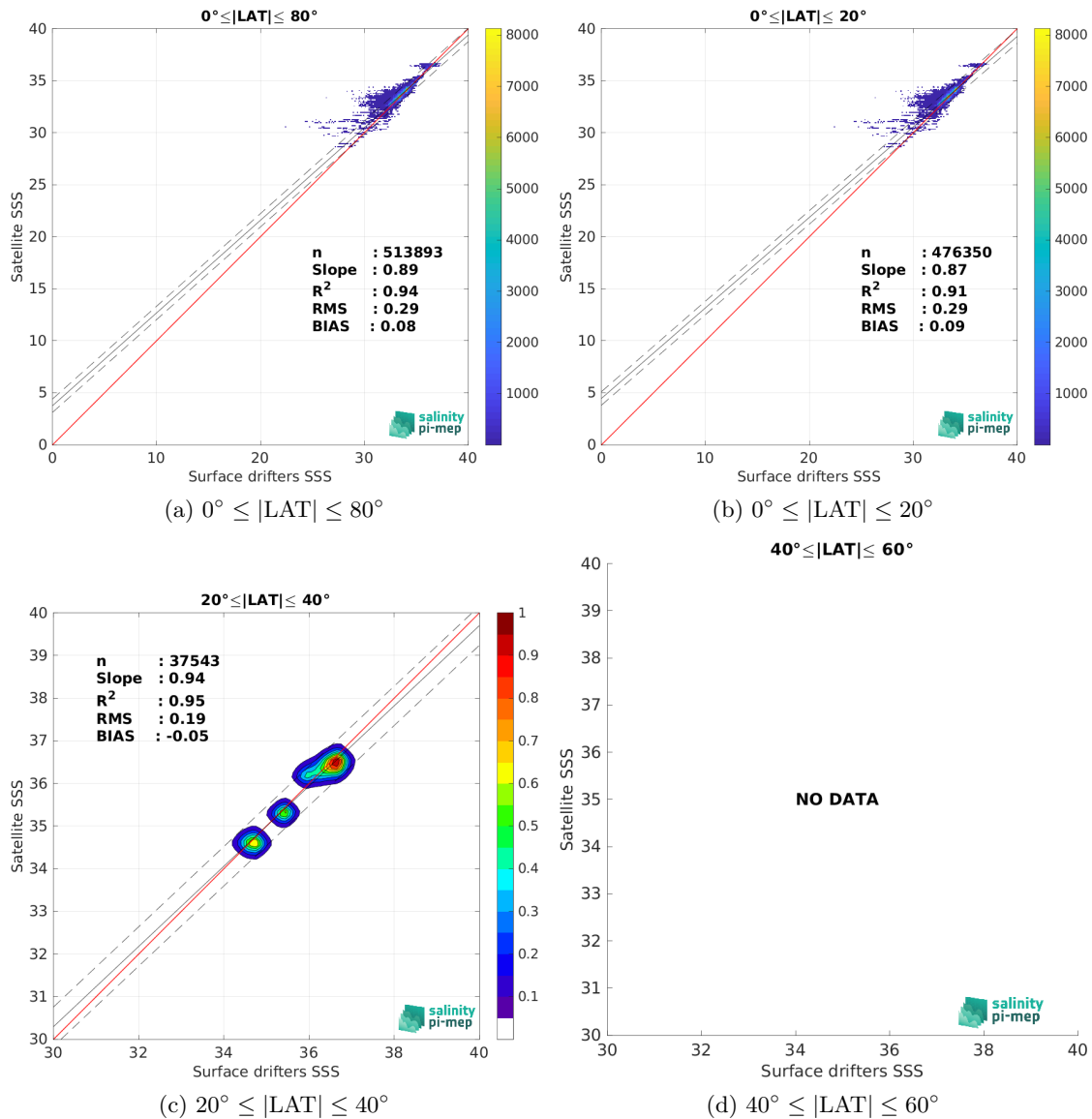
Figure 8: Contour maps of the concentration of SMAP SSS L4 OI v2 - Monthly (IPRC) SSS (y-axis) versus Surface drifters SSS (x-axis) at match-up pairs for different latitude (IPRC) bands. For each plot, the red line shows x=y . The black thin and dashed lines indicate a linear fit through the data cloud and the \pm 95\% confidence levels, respectively. The number match-up pairs n , the slope and R^2 coefficient of the linear fit, the root mean square (RMS) and the mean bias between satellite and in situ data are indicated for each latitude band in each plots.
