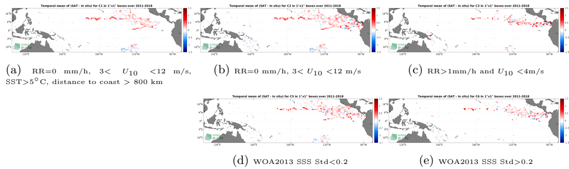
Figure 11: Temporal mean gridded over spatial boxes of size 1^\circ \times 1^\circ of \Delta SSS (SMAP SSS L4 OI v2 - Monthly (IPRC) - Surface drifters) for 5 different subdatasets corresponding to:RR=0 mm/h, 3 < U_{10} < 12 m/s, SST > 5^\circ\text{C} , distance to coast > 800 km (a), RR=0 mm/h, 3 < U_{10} < 12 m/s (b), RR > 1 mm/h and U_{10} < 4 m/s (c), WOA2013 SSS Std < 0.2 (d), WOA2013 SSS Std > 0.2 (e).
