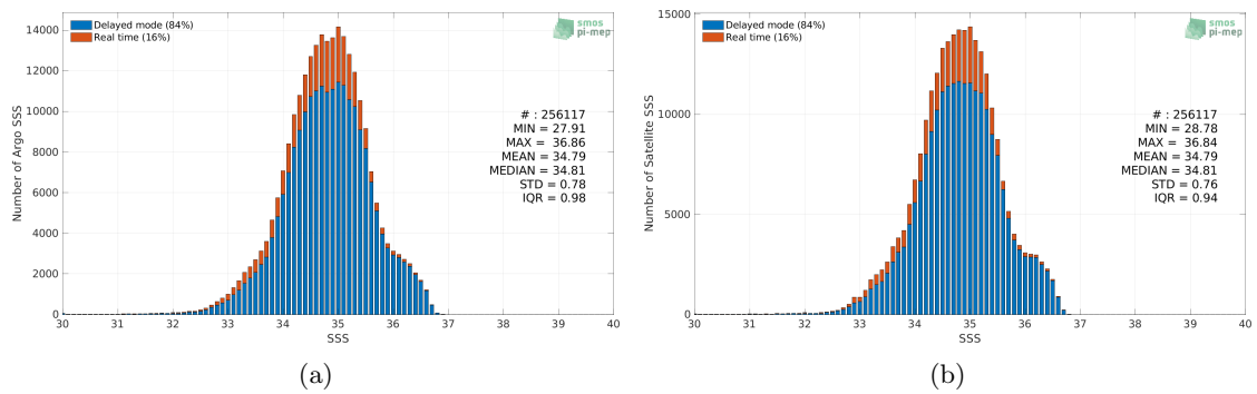
Figure 2: Histograms of SSS from Argo (a) and SMAP SSS L4 OI v2 - Monthly (IPRC) (b) considering all match-up pairs per bins of 0.1 over the Tropical Pacific Ocean Pi-MEP region and for the full satellite product period.
