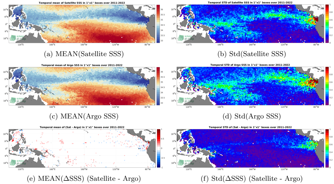
Figure 6: Temporal mean (left) and Std (right) of SSS from SMAP SSS L4 OI v2 - Monthly (IPRC) (top), Argo (middle), and of \Delta SSS (Satellite - Argo). Only match-up pairs are used to generate these maps.
