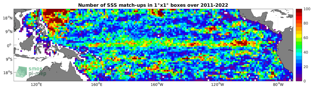
Figure 4: Number of SSS match-ups between Argo SSS and the SMAP SSS L4 OI v2 - Monthly (IPRC) SSS product for the Tropical Pacific Ocean Pi-MEP region over 1^\circ \times 1^\circ boxes and for the full satellite product period.
