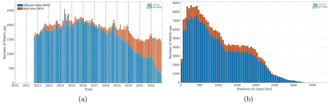
Figure 1: Number of match-ups between Argo and SMAP SSS L4 OI v2 - Monthly (IPRC) SSS as a function of time (a) and as function of the distance to coast (b) over the Tropical Pacific Ocean Pi-MEP region and for the full satellite product period.
