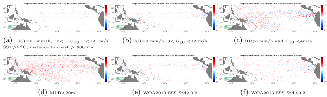
Figure 12: Temporal mean gridded over spatial boxes of size 1^\circ \times 1^\circ of \Delta SSS (SMAP SSS L4 OI v2 - Monthly (IPRC) - Argo) for 6 different subdatasets corresponding to:RR=0 mm/h, 3 < U_{10} < 12 m/s, SST >5^\circ C, distance to coast > 800 km (a), RR=0 mm/h, 3 < U_{10} < 12 m/s (b), RR >1 mm/h and U_{10} < 4 m/s (c),MLD <20 m (d),WOA2013 SSS Std <0.2 (e),WOA2013 SSS Std >0.2 (f).
