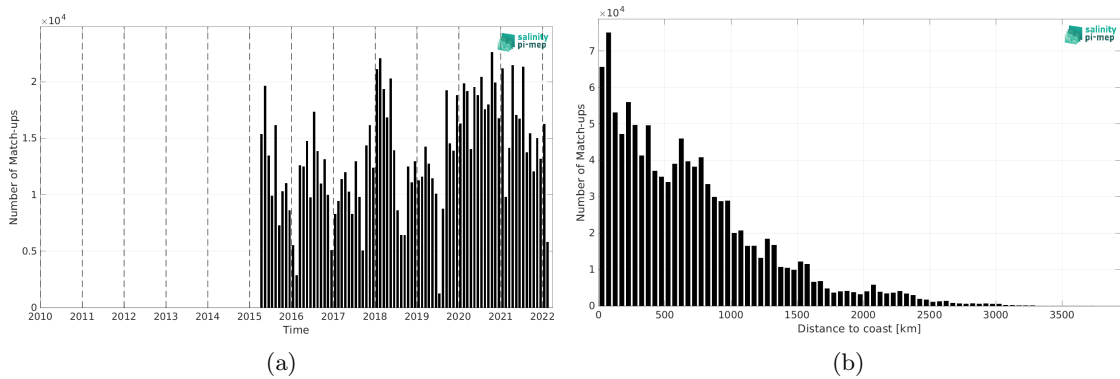
Figure 2: Number of match-ups between TSG (LEGOS-DM) and SMAP SSS L3 v6 - 8-Day running (RSS) SSS as a function of time (a) and as function of the distance to coast (b) over the Tropical Pacific Ocean Pi-MEP region and for the full satellite product period.
