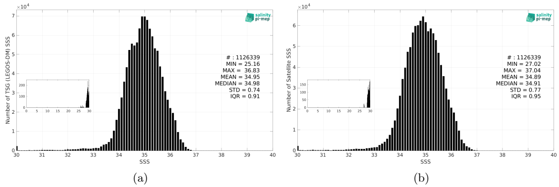
Figure 3: Histograms of SSS from TSG (LEGOS-DM) (a) and SMAP SSS L3 v6 - 8-Day running (RSS) (b) considering all match-up pairs per bins of 0.1 over the Tropical Pacific Ocean Pi-MEP region and for the full satellite product period.
