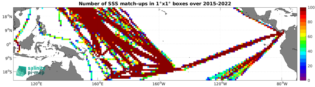
Figure 5: Number of SSS match-ups between TSG (LEGOS-DM) SSS and the SMAP SSS L3 v6 - 8-Day running (RSS) SSS product for the Tropical Pacific Ocean Pi-MEP region over 1^\circ \times 1^\circ boxes and for the full satellite product period.
