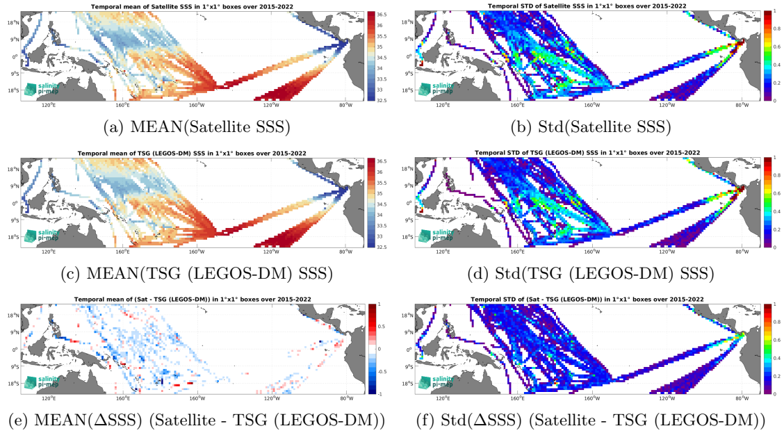
Figure 7: Temporal mean (left) and Std (right) of SSS from SMAP SSS L3 v6 - 8-Day running (RSS) (top), TSG (LEGOS-DM) (middle), and of \Delta SSS (Satellite - TSG (LEGOS-DM)). Only match-up pairs are used to generate these maps.
