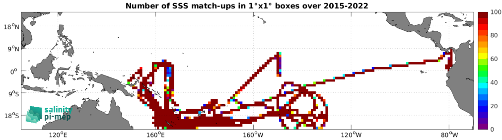
Figure 5: Number of SSS match-ups between TSG (GOSUD-Research-vessel) SSS and the SMAP SSS L3 v6 - 8-Day running (RSS) SSS product for the Tropical Pacific Ocean Pi-MEP region over 1^\circ \times 1^\circ boxes and for the full satellite product period.
