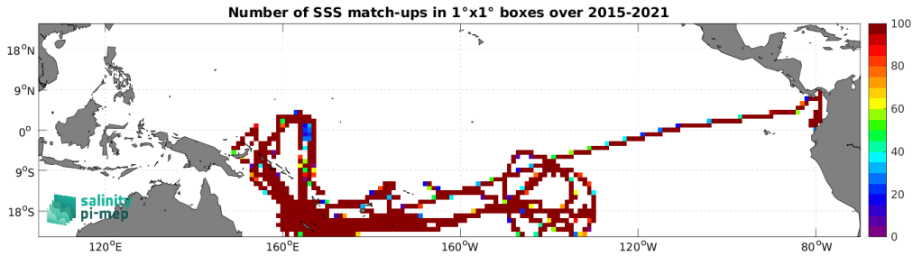
Figure 5: Number of SSS match-ups between TSG (GOSUD-Research-vessel) SSS and the SMAP SSS L3 v6 - 8-Day running (RSS) SSS product for the Tropical Pacific Ocean Pi-MEP region over 1^\circ \times 1^\circ boxes and for the full satellite product period.
