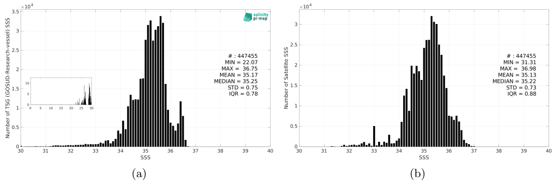
Figure 3: Histograms of SSS from TSG (GOSUD-Research-vessel) (a) and SMAP SSS L3 v6 - 8-Day running (RSS) (b) considering all match-up pairs per bins of 0.1 over the Tropical Pacific Ocean Pi-MEP region and for the full satellite product period.
