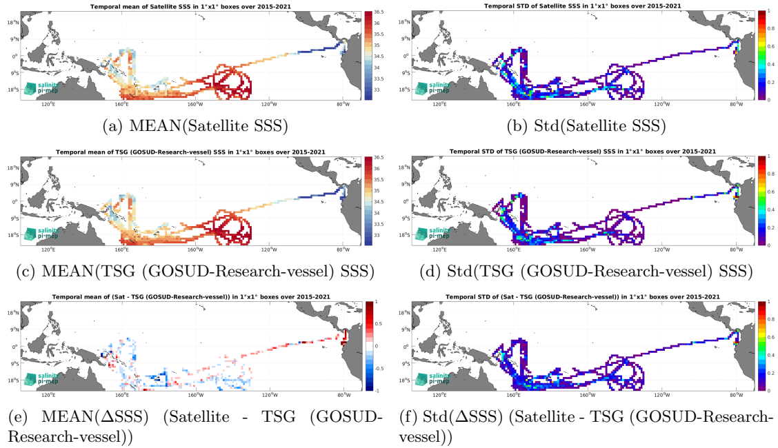
Figure 7: Temporal mean (left) and Std (right) of SSS from SMAP SSS L3 v6 - 8-Day running (RSS) (top), TSG (GOSUD-Research-vessel) (middle), and of \Delta SSS (Satellite - TSG (GOSUD-Research-vessel)). Only match-up pairs are used to generate these maps.
