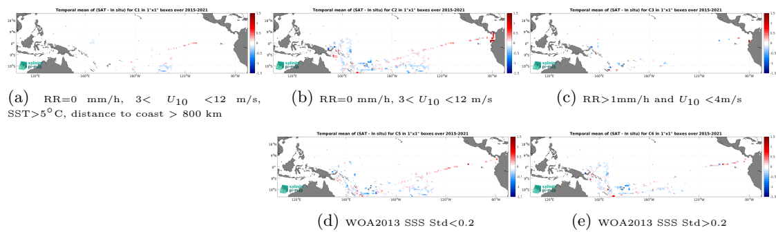
Figure 14: Temporal mean gridded over spatial boxes of size 1^\circ \times 1^\circ of \Delta SSS (SMAP SSS L3 v6 - 8-Day running (RSS) - TSG (GOSUD-Research-vessel)) for 5 different subdatasets corresponding to:RR=0 mm/h, 3 < U_{10} < 12 m/s, SST >5^\circ C, distance to coast > 800 km (a), RR=0 mm/h, 3 < U_{10} < 12 m/s (b), RR >1 mm/h and U_{10} < 4 m/s (c), WOA2013 SSS Std <0.2 (d), WOA2013 SSS Std >0.2 (e).
