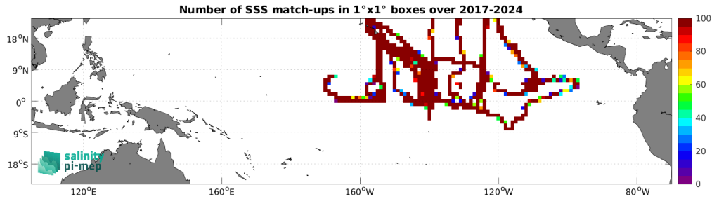
Figure 5: Number of SSS match-ups between Saildrone SSS and the SMAP SSS L3 v6 - 8-Day running (RSS) SSS product for the Tropical Pacific Ocean Pi-MEP region over 1^\circ \times 1^\circ boxes and for the full satellite product period.
