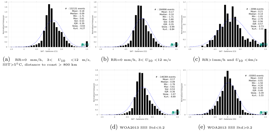
Figure 15: Normalized histogram of \Delta SSS (SMAP SSS L3 v6 - 8-Day running (RSS) - Saldrone) for 5 different subdatasets corresponding to: RR=0 mm/h, 3 < U_{10} < 12 m/s, SST>5°C, distance to coast > 800 km (a), RR=0 mm/h, 3 < U_{10} < 12 m/s (b), RR>1mm/h and U_{10} < 4 m/s (c), WOA2013 SSS Std<0.2 (d), WOA2013 SSS Std>0.2 (e).
