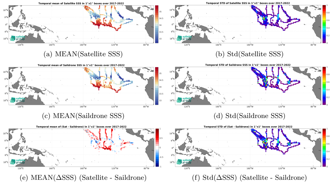
Figure 7: Temporal mean (left) and Std (right) of SSS from SMAP SSS L3 v6 - 8-Day running (RSS) (top), Saildrone (middle), and of \Delta SSS (Satellite - Saildrone). Only match-up pairs are used to generate these maps.
