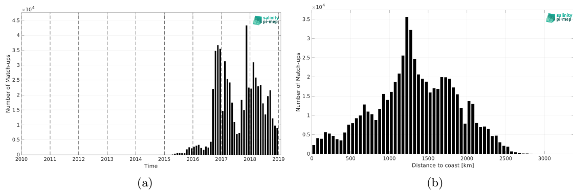
Figure 2: Number of match-ups between Surface drifters and SMAP SSS L3 v6 - 8-Day running (RSS) SSS as a function of time (a) and as function of the distance to coast (b) over the Tropical Pacific Ocean Pi-MEP region and for the full satellite product period.
