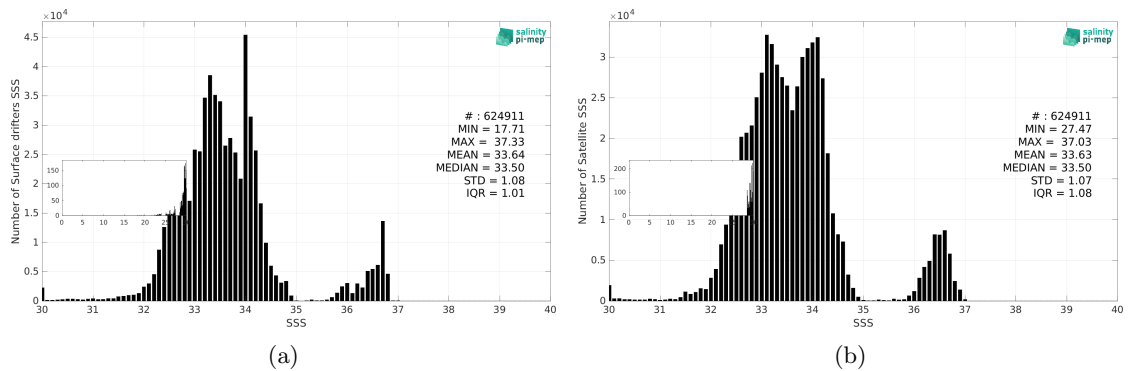
Figure 3: Histograms of SSS from Surface drifters (a) and SMAP SSS L3 v6 - 8-Day running (RSS) (b) considering all match-up pairs per bins of 0.1 over the Tropical Pacific Ocean Pi-MEP region and for the full satellite product period.
