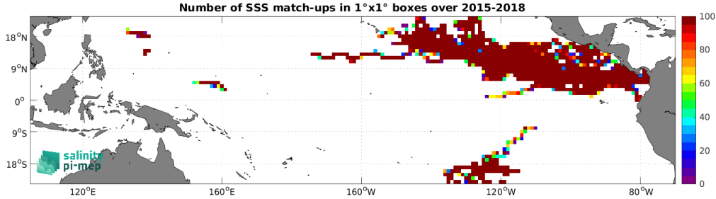
Figure 4: Number of SSS match-ups between Surface drifters SSS and the SMAP SSS L3 v6 - 8-Day running (RSS) SSS product for the Tropical Pacific Ocean Pi-MEP region over 1^\circ \times 1^\circ boxes and for the full satellite product period.
