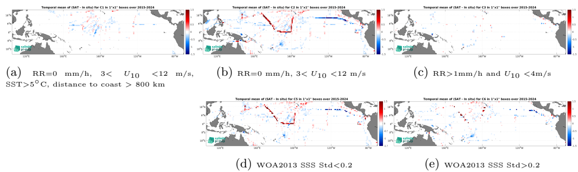
Figure 14: Temporal mean gridded over spatial boxes of size 1^\circ \times 1^\circ of \Delta SSS (SMAP SSS L3 v6 - Monthly (RSS) - TSG (SAMOS)) for 5 different subdatasets corresponding to:RR=0 mm/h, 3 < U_{10} < 12 m/s, SST >5^\circ C, distance to coast > 800 km (a), RR=0 mm/h, 3 < U_{10} < 12 m/s (b), RR >1 mm/h and U_{10} < 4 m/s (c), WOA2013 SSS Std <0.2 (d), WOA2013 SSS Std >0.2 (e).
