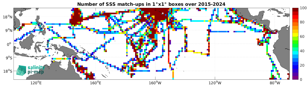
Figure 5: Number of SSS match-ups between TSG (SAMOS) SSS and the SMAP SSS L3 v6 - Monthly (RSS) SSS product for the Tropical Pacific Ocean Pi-MEP region over 1^\circ \times 1^\circ boxes and for the full satellite product period.
