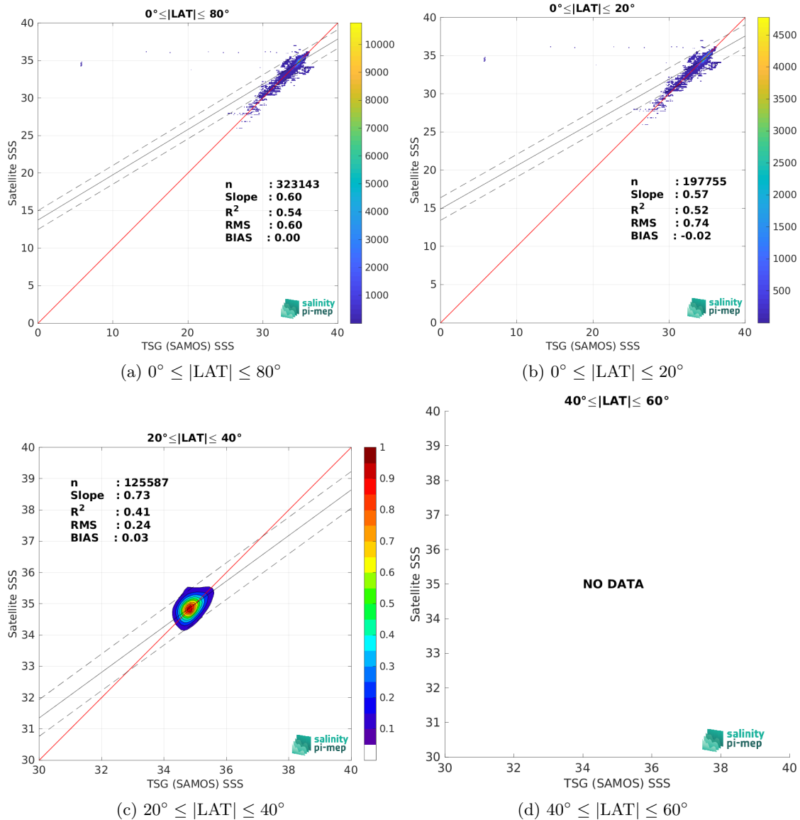
Figure 10: Contour maps of the concentration of SMAP SSS L3 v6 - Monthly (RSS) SSS (y-axis) versus TSG (SAMOS) SSS (x-axis) at match-up pairs for different latitude bands. For each plot, the red line shows x=y . The black thin and dashed lines indicate a linear fit through the data cloud and the \pm 95\% confidence levels, respectively. The number match-up pairs n , the slope and R^2 coefficient of the linear fit, the root mean square (RMS) and the mean bias between satellite and in situ data are indicated for each latitude band in each plots.
