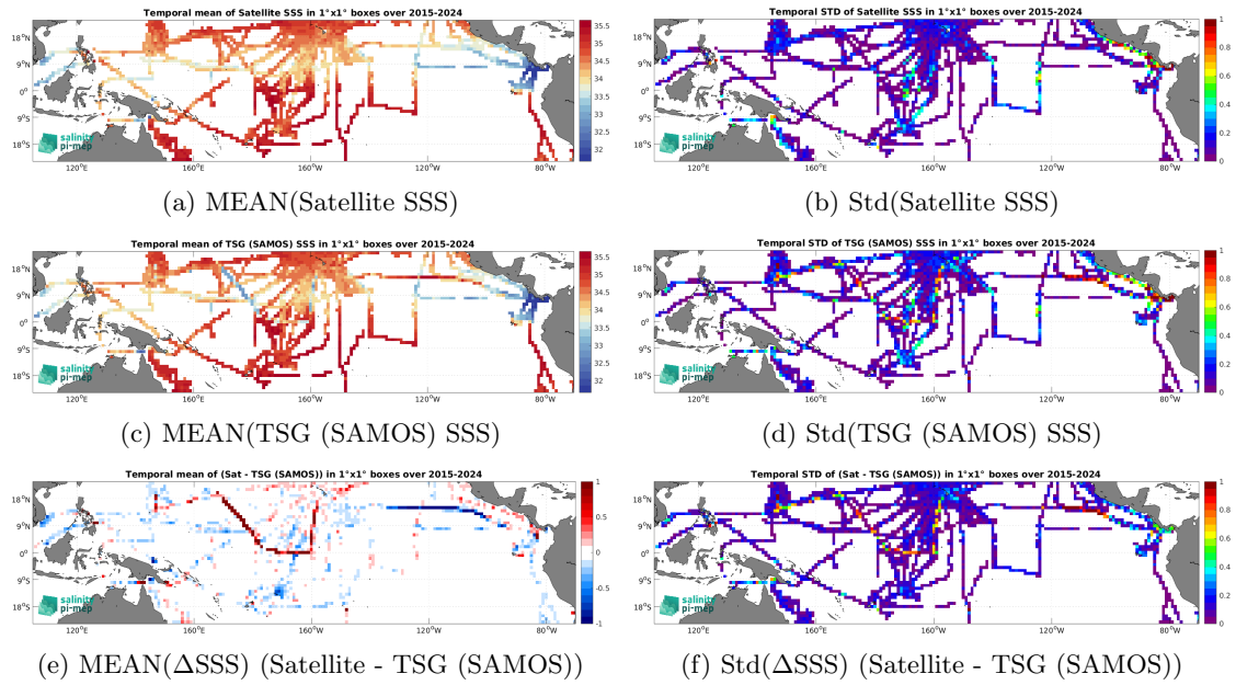
Figure 7: Temporal mean (left) and Std (right) of SSS from SMAP SSS L3 v6 - Monthly (RSS) (top), TSG (SAMOS) (middle), and of \Delta SSS (Satellite - TSG (SAMOS)). Only match-up pairs are used to generate these maps.
