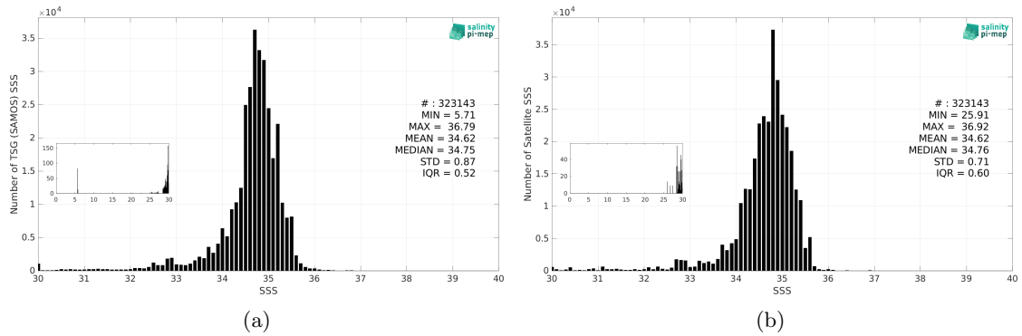
Figure 3: Histograms of SSS from TSG (SAMOS) (a) and SMAP SSS L3 v6 - Monthly (RSS) (b) considering all match-up pairs per bins of 0.1 over the Tropical Pacific Ocean Pi-MEP region and for the full satellite product period.
