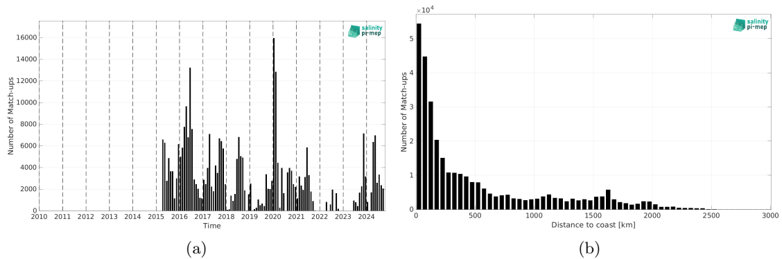
Figure 2: Number of match-ups between TSG (SAMOS) and SMAP SSS L3 v6 - Monthly (RSS) SSS as a function of time (a) and as function of the distance to coast (b) over the Tropical Pacific Ocean Pi-MEP region and for the full satellite product period.
