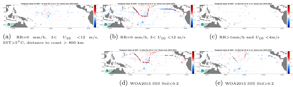
Figure 14: Temporal mean gridded over spatial boxes of size 1^\circ \times 1^\circ of \Delta\text{SSS} (SMAP SSS L3 v6 - Monthly (RSS) - TSG (SAMOS)) for 5 different subdatasets corresponding to:RR=0 mm/h, 3 < U_{10} < 12 m/s, SST > 5^\circ\text{C} , distance to coast > 800 km (a), RR=0 mm/h, 3 < U_{10} < 12 m/s (b), RR > 1 mm/h and U_{10} < 4 m/s (c), WOA2013 SSS Std < 0.2 (d), WOA2013 SSS Std > 0.2 (e).
