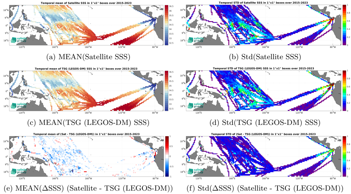
Figure 7: Temporal mean (left) and Std (right) of SSS from SMAP SSS L3 v6 - Monthly (RSS) (top), TSG (LEGOS-DM) (middle), and of \Delta SSS (Satellite - TSG (LEGOS-DM)). Only match-up pairs are used to generate these maps.
