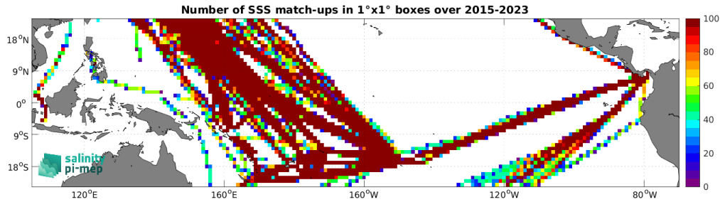
Figure 5: Number of SSS match-ups between TSG (LEGOS-DM) SSS and the SMAP SSS L3 v6 - Monthly (RSS) SSS product for the Tropical Pacific Ocean Pi-MEP region over 1^\circ \times 1^\circ boxes and for the full satellite product period.
