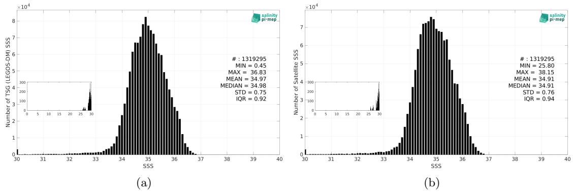
Figure 3: Histograms of SSS from TSG (LEGOS-DM) (a) and SMAP SSS L3 v6 - Monthly (RSS) (b) considering all match-up pairs per bins of 0.1 over the Tropical Pacific Ocean Pi-MEP region and for the full satellite product period.
