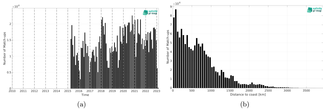
Figure 2: Number of match-ups between TSG (LEGOS-DM) and SMAP SSS L3 v6 - Monthly (RSS) SSS as a function of time (a) and as function of the distance to coast (b) over the Tropical Pacific Ocean Pi-MEP region and for the full satellite product period.
