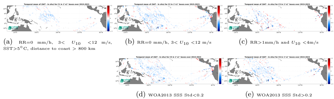
Figure 14: Temporal mean gridded over spatial boxes of size 1^\circ \times 1^\circ of \Delta SSS (SMAP SSS L3 v6 - Monthly (RSS) - TSG (LEGOS-DM)) for 5 different subdatasets corresponding to: RR=0 mm/h, 3 < U_{10} < 12 m/s, SST > 5^\circ\text{C} , distance to coast > 800 km (a), RR=0 mm/h, 3 < U_{10} < 12 m/s (b), RR > 1 mm/h and U_{10} < 4 m/s (c), WOA2013 SSS Std < 0.2 (d), WOA2013 SSS Std > 0.2 (e).
