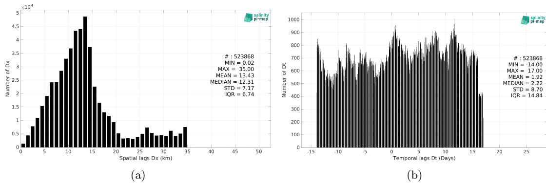
Figure 6: Histograms of the spatial (a) and temporal (b) lags between the location/time of the TSG (GOSUD-Research-vessel) measurement and the date of the corresponding SMAP SSS L3 v6 - Monthly (RSS) SSS pixel.
