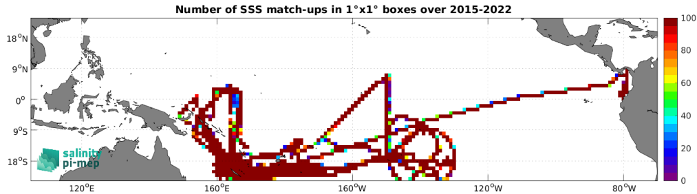
Figure 5: Number of SSS match-ups between TSG (GOSUD-Research-vessel) SSS and the SMAP SSS L3 v6 - Monthly (RSS) SSS product for the Tropical Pacific Ocean Pi-MEP region over 1^\circ \times 1^\circ boxes and for the full satellite product period.
