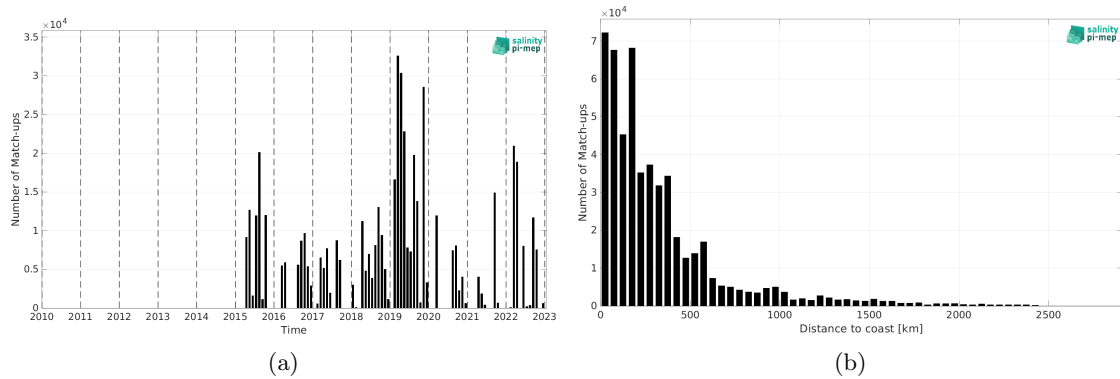
Figure 2: Number of match-ups between TSG (GOSUD-Research-vessel) and SMAP SSS L3 v6 - Monthly (RSS) SSS as a function of time (a) and as function of the distance to coast (b) over the Tropical Pacific Ocean Pi-MEP region and for the full satellite product period.
