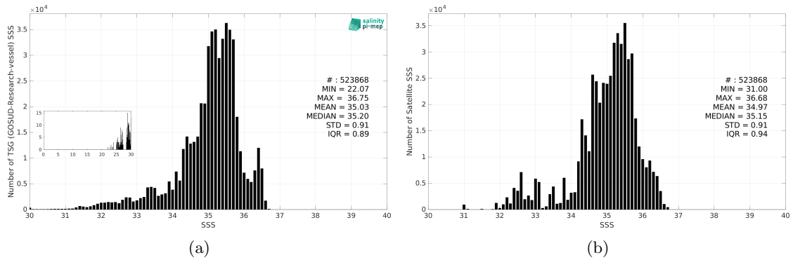
Figure 3: Histograms of SSS from TSG (GOSUD-Research-vessel) (a) and SMAP SSS L3 v6 - Monthly (RSS) (b) considering all match-up pairs per bins of 0.1 over the Tropical Pacific Ocean Pi-MEP region and for the full satellite product period.
