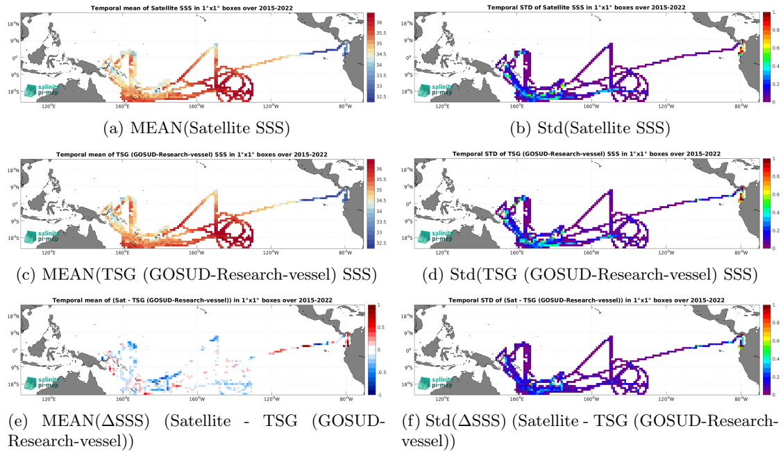
Figure 7: Temporal mean (left) and Std (right) of SSS from SMAP SSS L3 v6 - Monthly (RSS) (top), TSG (GOSUD-Research-vessel) (middle), and of \Delta SSS (Satellite - TSG (GOSUD-Research-vessel)). Only match-up pairs are used to generate these maps.
