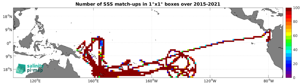
Figure 5: Number of SSS match-ups between TSG (GOSUD-Research-vessel) SSS and the SMAP SSS L3 v6 - Monthly (RSS) SSS product for the Tropical Pacific Ocean Pi-MEP region over 1^\circ \times 1^\circ boxes and for the full satellite product period.
