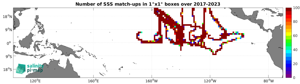
Figure 5: Number of SSS match-ups between Saildrone SSS and the SMAP SSS L3 v6 - Monthly (RSS) SSS product for the Tropical Pacific Ocean Pi-MEP region over 1^\circ \times 1^\circ boxes and for the full satellite product period.
