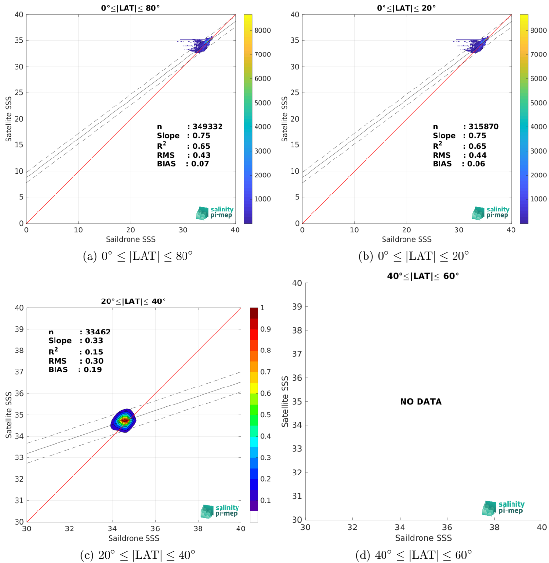
Figure 10: Contour maps of the concentration of SMAP SSS L3 v6 - Monthly (RSS) SSS (y-axis) versus Sairdron SSS (x-axis) at match-up pairs for different latitude bands. For each plot, the red line shows x=y . The black thin and dashed lines indicate a linear fit through the data cloud and the \pm 95\% confidence levels, respectively. The number match-up pairs n , the slope and R^2 coefficient of the linear fit, the root mean square (RMS) and the mean bias between satellite and in situ data are indicated for each latitude band in each plots.
