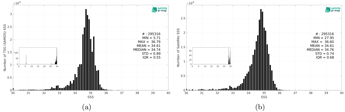
Figure 3: Histograms of SSS from TSG (SAMOS) (a) and SMAP SSS L3 v5.3 - 8-Day running (RSS) (b) considering all match-up pairs per bins of 0.1 over the Tropical Pacific Ocean Pi-MEP region and for the full satellite product period.
