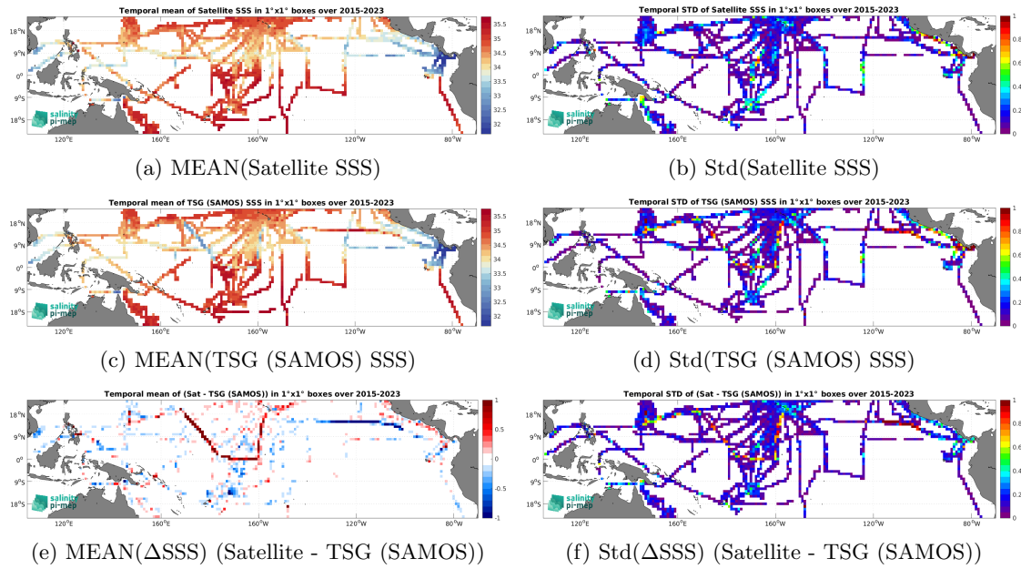
Figure 7: Temporal mean (left) and Std (right) of SSS from SMAP SSS L3 v5.3 - 8-Day running (RSS) (top), TSG (SAMOS) (middle), and of \Delta SSS (Satellite - TSG (SAMOS)). Only match-up pairs are used to generate these maps.
