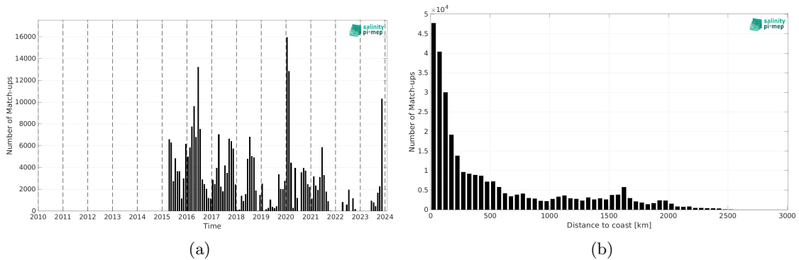
Figure 2: Number of match-ups between TSG (SAMOS) and SMAP SSS L3 v5.3 - 8-Day running (RSS) SSS as a function of time (a) and as function of the distance to coast (b) over the Tropical Pacific Ocean Pi-MEP region and for the full satellite product period.
