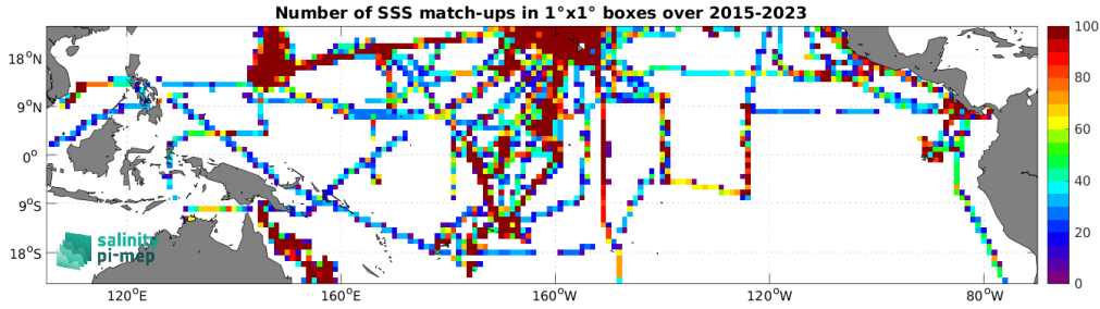
Figure 5: Number of SSS match-ups between TSG (SAMOS) SSS and the SMAP SSS L3 v5.3 - 8-Day running (RSS) SSS product for the Tropical Pacific Ocean Pi-MEP region over 1^\circ \times 1^\circ boxes and for the full satellite product period.
