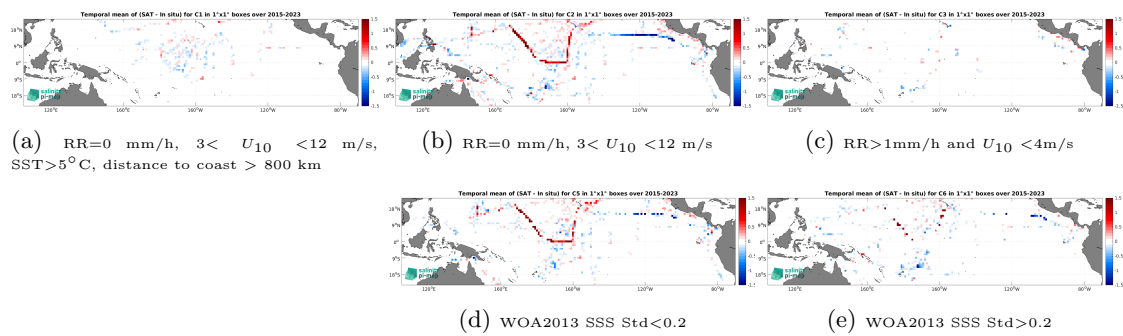
Figure 14: Temporal mean gridded over spatial boxes of size 1^\circ \times 1^\circ of \Delta SSS (SMAP SSS L3 v5.3 - 8-Day running (RSS) - TSG (SAMOS)) for 5 different subdatasets corresponding to: RR=0 mm/h, 3 < U_{10} < 12 m/s, SST > 5^\circ\text{C} , distance to coast > 800 km (a), RR=0 mm/h, 3 < U_{10} < 12 m/s (b), RR > 1 mm/h and U_{10} < 4 m/s (c), WOA2013 SSS Std < 0.2 (d), WOA2013 SSS Std > 0.2 (e).
