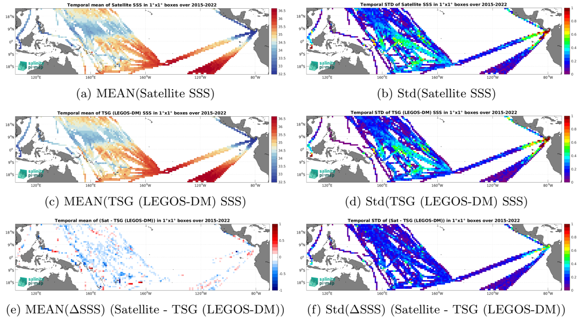
Figure 7: Temporal mean (left) and Std (right) of SSS from SMAP SSS L3 v5.3 - 8-Day running (RSS) (top), TSG (LEGOS-DM) (middle), and of \Delta SSS (Satellite - TSG (LEGOS-DM)). Only match-up pairs are used to generate these maps.
