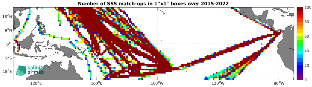
Figure 5: Number of SSS match-ups between TSG (LEGOS-DM) SSS and the SMAP SSS L3 v5.3 - 8-Day running (RSS) SSS product for the Tropical Pacific Ocean Pi-MEP region over 1^\circ \times 1^\circ boxes and for the full satellite product period.
