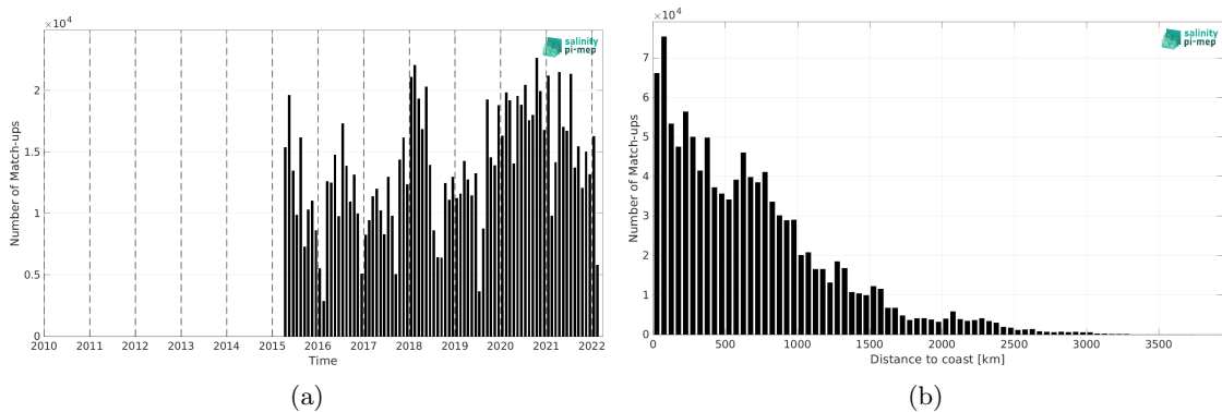
Figure 2: Number of match-ups between TSG (LEGOS-DM) and SMAP SSS L3 v5.3 - 8-Day running (RSS) SSS as a function of time (a) and as function of the distance to coast (b) over the Tropical Pacific Ocean Pi-MEP region and for the full satellite product period.
