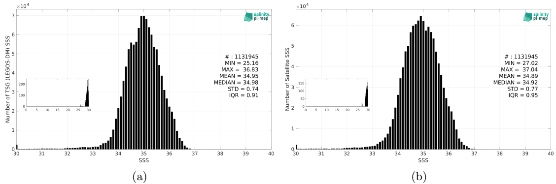
Figure 3: Histograms of SSS from TSG (LEGOS-DM) (a) and SMAP SSS L3 v5.3 - 8-Day running (RSS) (b) considering all match-up pairs per bins of 0.1 over the Tropical Pacific Ocean Pi-MEP region and for the full satellite product period.
