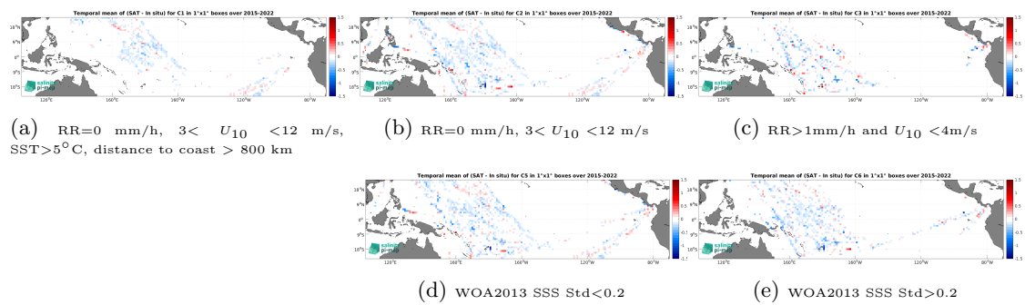
Figure 14: Temporal mean gridded over spatial boxes of size 1^\circ \times 1^\circ of \Delta SSS (SMAP SSS L3 v5.3 - 8-Day running (RSS) - TSG (LEGOS-DM)) for 5 different subdatasets corresponding to: RR=0 mm/h, 3 < U_{10} < 12 m/s, SST > 5^\circ\text{C} , distance to coast > 800 km (a), RR=0 mm/h, 3 < U_{10} < 12 m/s (b), RR > 1 mm/h and U_{10} < 4 m/s (c), WOA2013 SSS Std < 0.2 (d), WOA2013 SSS Std > 0.2 (e).
