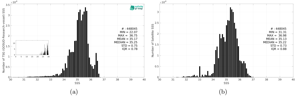
Figure 3: Histograms of SSS from TSG (GOSUD-Research-vessel) (a) and SMAP SSS L3 v5.3 - 8-Day running (RSS) (b) considering all match-up pairs per bins of 0.1 over the Tropical Pacific Ocean Pi-MEP region and for the full satellite product period.
