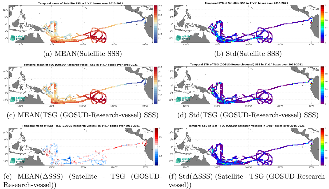
Figure 7: Temporal mean (left) and Std (right) of SSS from SMAP SSS L3 v5.3 - 8-Day running (RSS) (top), TSG (GOSUD-Research-vessel) (middle), and of \Delta SSS (Satellite - TSG (GOSUD-Research-vessel)). Only match-up pairs are used to generate these maps.
