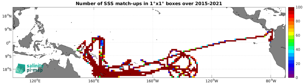
Figure 5: Number of SSS match-ups between TSG (GOSUD-Research-vessel) SSS and the SMAP SSS L3 v5.3 - 8-Day running (RSS) SSS product for the Tropical Pacific Ocean Pi-MEP region over 1^\circ \times 1^\circ boxes and for the full satellite product period.
