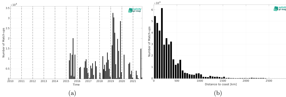
Figure 2: Number of match-ups between TSG (GOSUD-Research-vessel) and SMAP SSS L3 v5.3 - 8-Day running (RSS) SSS as a function of time (a) and as function of the distance to coast (b) over the Tropical Pacific Ocean Pi-MEP region and for the full satellite product period.
