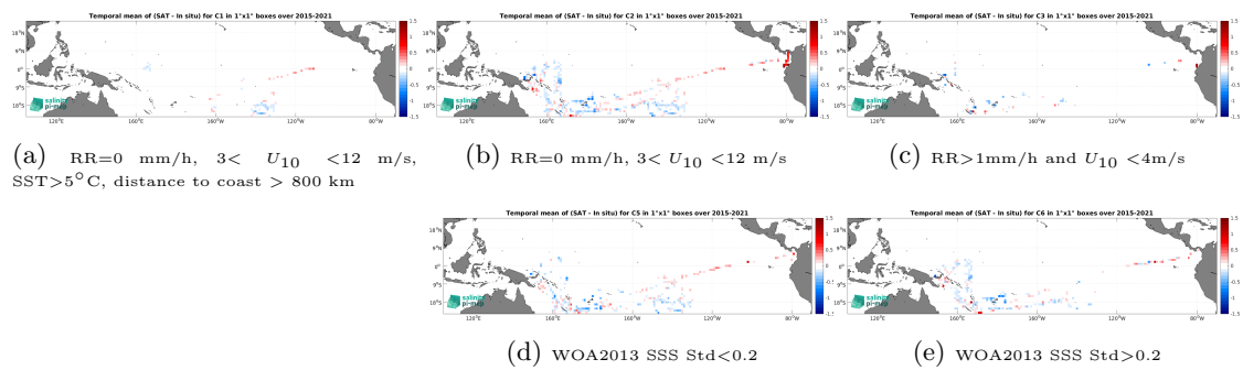
Figure 14: Temporal mean gridded over spatial boxes of size 1^\circ \times 1^\circ of \Delta SSS (SMAP SSS L3 v5.3 - 8-Day running (RSS) - TSG (GOSUD-Research-vessel)) for 5 different subdatasets corresponding to:RR=0 mm/h, 3 < U_{10} < 12 m/s, SST > 5^\circ\text{C} , distance to coast > 800 km (a), RR=0 mm/h, 3 < U_{10} < 12 m/s (b), RR > 1 mm/h and U_{10} < 4 m/s (c), WOA2013 SSS Std < 0.2 (d), WOA2013 SSS Std > 0.2 (e).
