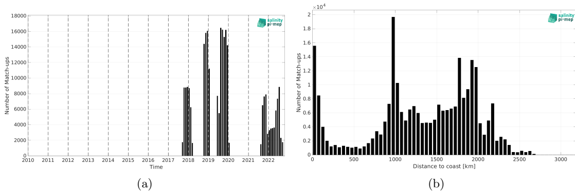
Figure 2: Number of match-ups between Saildrone and SMAP SSS L3 v5.3 - 8-Day running (RSS) SSS as a function of time (a) and as function of the distance to coast (b) over the Tropical Pacific Ocean Pi-MEP region and for the full satellite product period.
