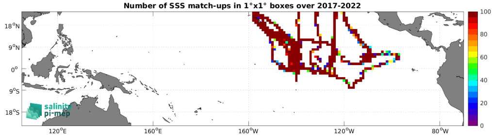
Figure 5: Number of SSS match-ups between Saildrone SSS and the SMAP SSS L3 v5.3 - 8-Day running (RSS) SSS product for the Tropical Pacific Ocean Pi-MEP region over 1^\circ \times 1^\circ boxes and for the full satellite product period.
