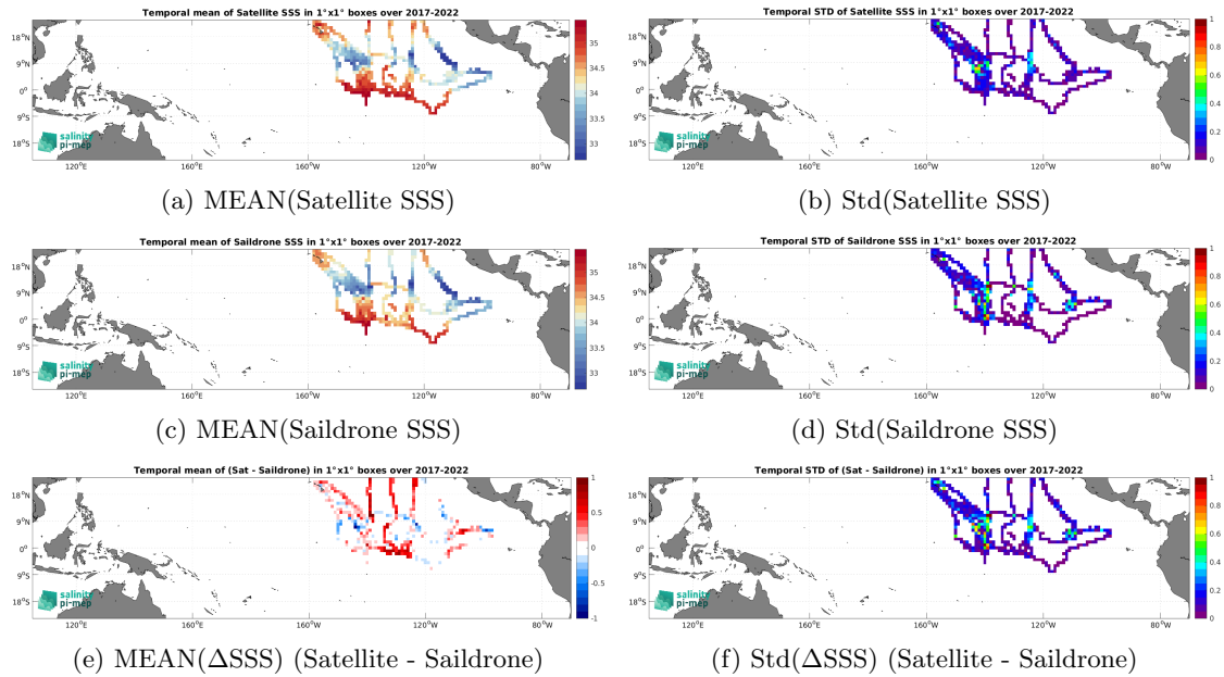
Figure 7: Temporal mean (left) and Std (right) of SSS from SMAP SSS L3 v5.3 - 8-Day running (RSS) (top), Saildrone (middle), and of \Delta SSS (Satellite - Saildrone). Only match-up pairs are used to generate these maps.
