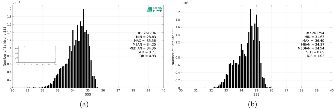
Figure 3: Histograms of SSS from Saildrone (a) and SMAP SSS L3 v5.3 - 8-Day running (RSS) (b) considering all match-up pairs per bins of 0.1 over the Tropical Pacific Ocean Pi-MEP region and for the full satellite product period.
