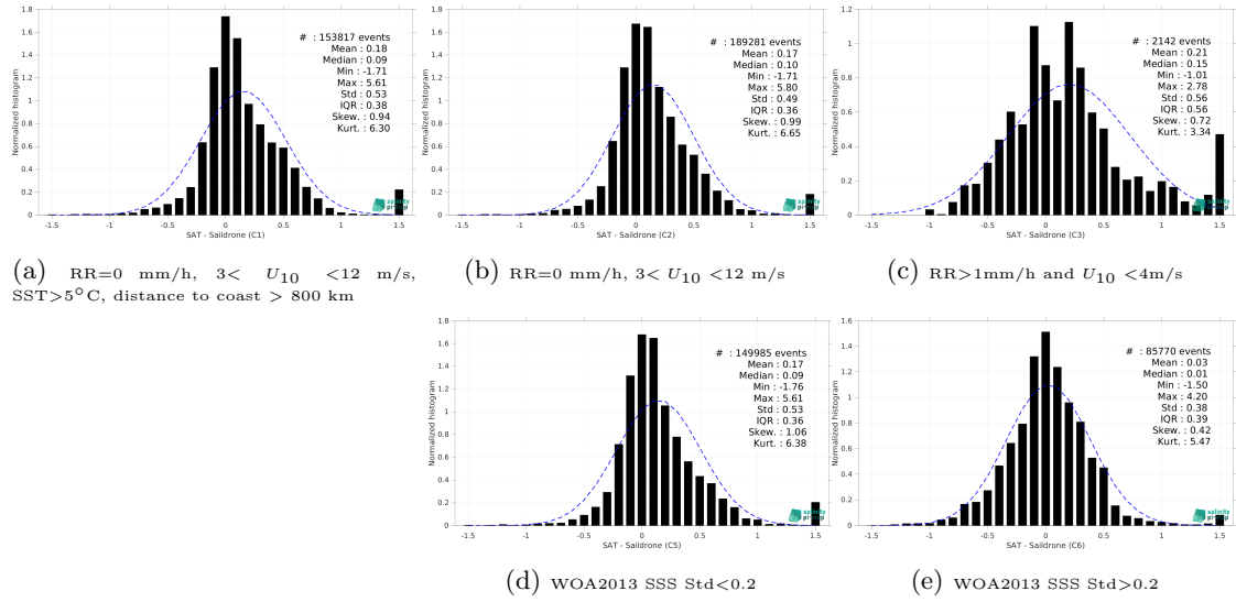
Figure 15: Normalized histogram of \Delta SSS (SMAP SSS L3 v5.3 - 8-Day running (RSS) - Saildrone) for 5 different subdatasets corresponding to: RR=0 mm/h, 3 < U_{10} < 12 m/s, SST>5°C, distance to coast > 800 km (a), RR=0 mm/h, 3 < U_{10} < 12 m/s (b), RR>1mm/h and U_{10} < 4 m/s (c), WOA2013 SSS Std<0.2 (d), WOA2013 SSS Std>0.2 (e).
