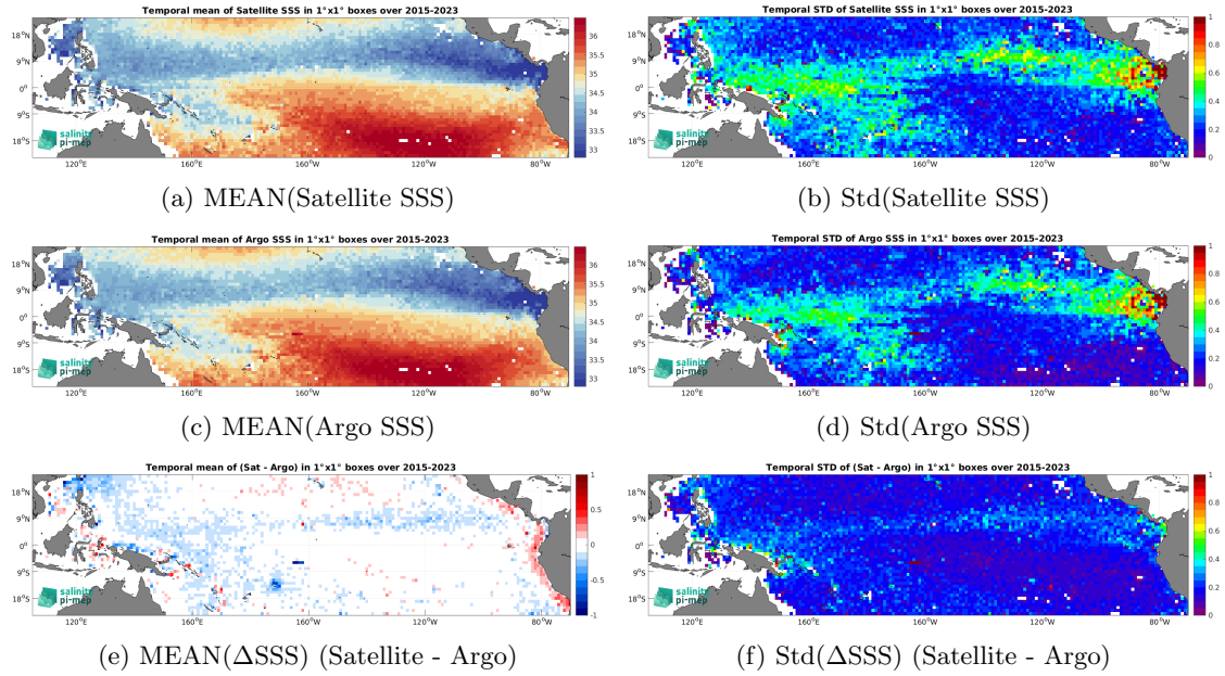
Figure 7: Temporal mean (left) and Std (right) of SSS from SMAP SSS L3 v5.3 - 8-Day running (RSS) (top), Argo (middle), and of \Delta SSS (Satellite - Argo). Only match-up pairs are used to generate these maps.
