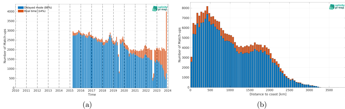
Figure 2: Number of match-ups between Argo and SMAP SSS L3 v5.3 - 8-Day running (RSS) SSS as a function of time (a) and as function of the distance to coast (b) over the Tropical Pacific Ocean Pi-MEP region and for the full satellite product period.
