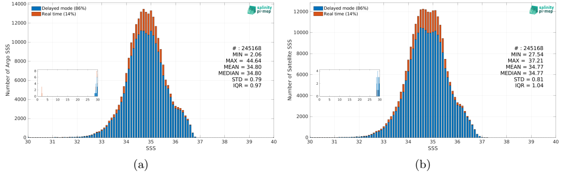
Figure 3: Histograms of SSS from Argo (a) and SMAP SSS L3 v5.3 - 8-Day running (RSS) (b) considering all match-up pairs per bins of 0.1 over the Tropical Pacific Ocean Pi-MEP region and for the full satellite product period.
