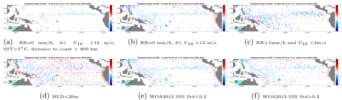
Figure 14: Temporal mean gridded over spatial boxes of size 1^\circ \times 1^\circ of \Delta SSS (SMAP SSS L3 v5.3 - 8-Day running (RSS) - Argo) for 6 different subdatasets corresponding to:RR=0 mm/h, 3 < U_{10} < 12 m/s, SST >5^\circ C, distance to coast > 800 km (a), RR=0 mm/h, 3 < U_{10} < 12 m/s (b), RR >1 mm/h and U_{10} < 4 m/s (c),MLD <20 m (d),WOA2013 SSS Std <0.2 (e),WOA2013 SSS Std >0.2 (f).
