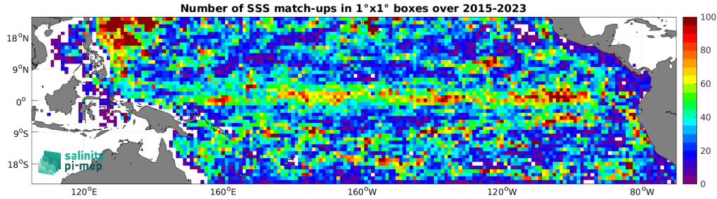
Figure 5: Number of SSS match-ups between Argo SSS and the SMAP SSS L3 v5.3 - 8-Day running (RSS) SSS product for the Tropical Pacific Ocean Pi-MEP region over 1^\circ \times 1^\circ boxes and for the full satellite product period.
