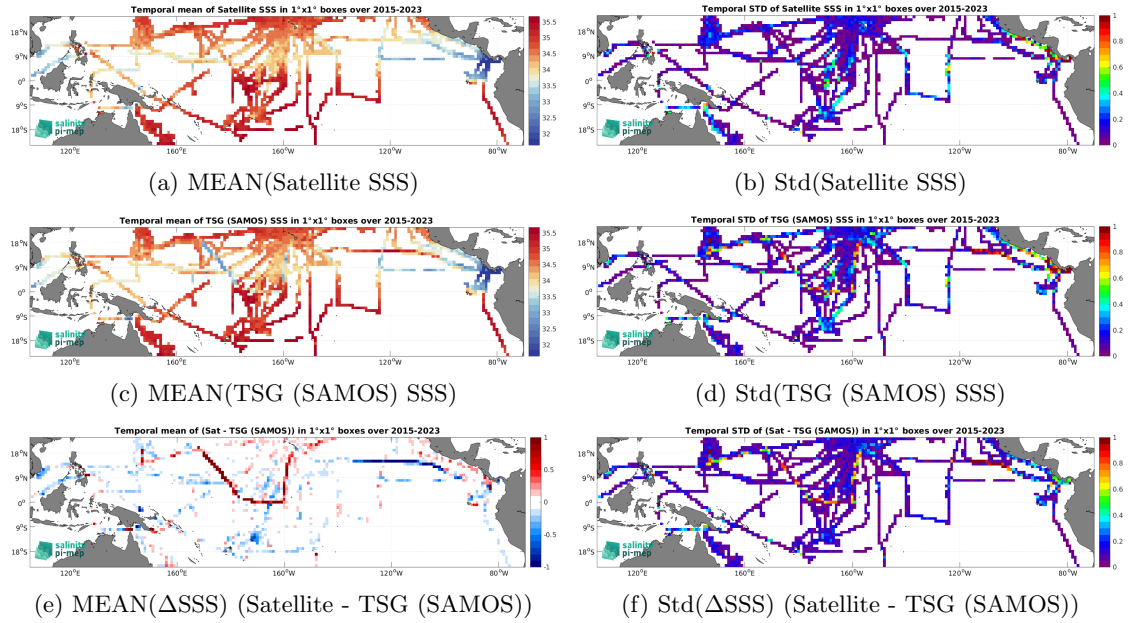
Figure 7: Temporal mean (left) and Std (right) of SSS from SMAP SSS L3 v5.3 - Monthly (RSS) (top), TSG (SAMOS) (middle), and of \Delta SSS (Satellite - TSG (SAMOS)). Only match-up pairs are used to generate these maps.
