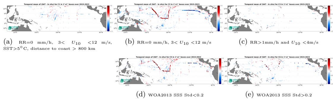
Figure 14: Temporal mean gridded over spatial boxes of size 1^\circ \times 1^\circ of \Delta SSS (SMAP SSS L3 v5.3 - Monthly (RSS) - TSG (SAMOS)) for 5 different subdatasets corresponding to:RR=0 mm/h, 3 < U_{10} < 12 m/s, SST >5^\circ C, distance to coast > 800 km (a), RR=0 mm/h, 3 < U_{10} < 12 m/s (b), RR >1 mm/h and U_{10} < 4 m/s (c), WOA2013 SSS Std <0.2 (d), WOA2013 SSS Std >0.2 (e).
