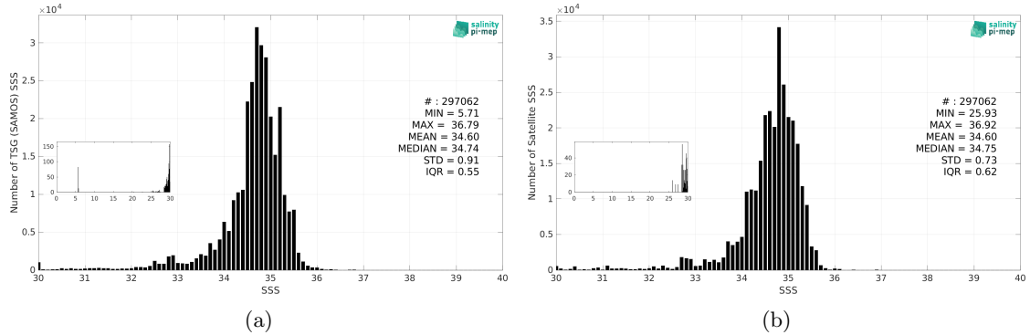
Figure 3: Histograms of SSS from TSG (SAMOS) (a) and SMAP SSS L3 v5.3 - Monthly (RSS) (b) considering all match-up pairs per bins of 0.1 over the Tropical Pacific Ocean Pi-MEP region and for the full satellite product period.
