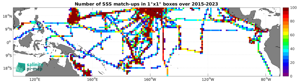
Figure 5: Number of SSS match-ups between TSG (SAMOS) SSS and the SMAP SSS L3 v5.3 - Monthly (RSS) SSS product for the Tropical Pacific Ocean Pi-MEP region over 1^\circ \times 1^\circ boxes and for the full satellite product period.
