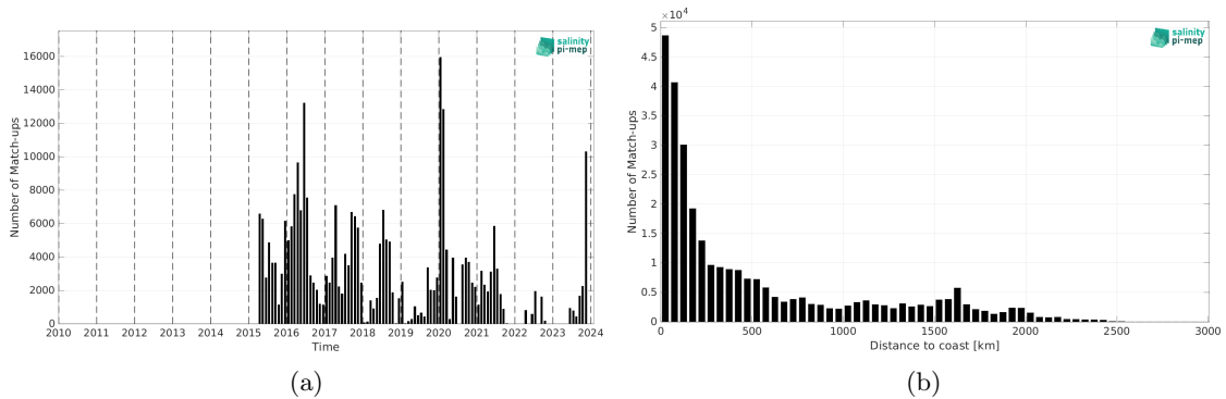
Figure 2: Number of match-ups between TSG (SAMOS) and SMAP SSS L3 v5.3 - Monthly (RSS) SSS as a function of time (a) and as function of the distance to coast (b) over the Tropical Pacific Ocean Pi-MEP region and for the full satellite product period.
