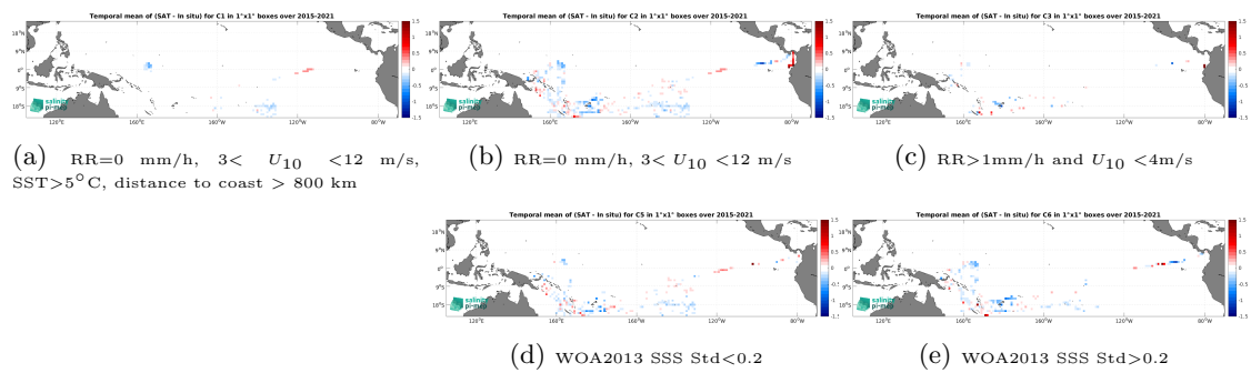
Figure 14: Temporal mean gridded over spatial boxes of size 1^\circ \times 1^\circ of \Delta SSS (SMAP SSS L3 v5.3 - Monthly (RSS) - TSG (GOSUD-Research-vessel)) for 5 different subdatasets corresponding to:RR=0 mm/h, 3 < U_{10} < 12 m/s, SST >5^\circ\text{C} , distance to coast > 800 km (a), RR=0 mm/h, 3 < U_{10} < 12 m/s (b), RR >1 mm/h and U_{10} < 4 m/s (c), WOA2013 SSS Std <0.2 (d), WOA2013 SSS Std >0.2 (e).
