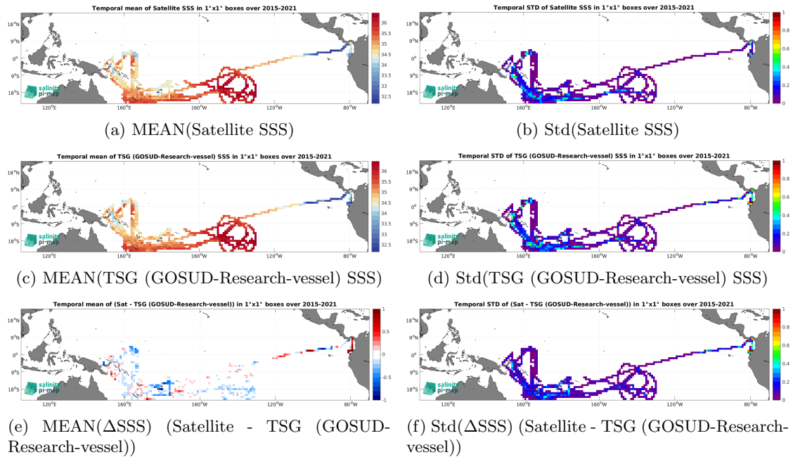
Figure 7: Temporal mean (left) and Std (right) of SSS from SMAP SSS L3 v5.3 - Monthly (RSS) (top), TSG (GOSUD-Research-vessel) (middle), and of \Delta SSS (Satellite - TSG (GOSUD-Research-vessel)). Only match-up pairs are used to generate these maps.
