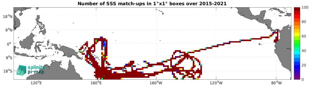
Figure 5: Number of SSS match-ups between TSG (GOSUD-Research-vessel) SSS and the SMAP SSS L3 v5.3 - Monthly (RSS) SSS product for the Tropical Pacific Ocean Pi-MEP region over 1^\circ \times 1^\circ boxes and for the full satellite product period.
