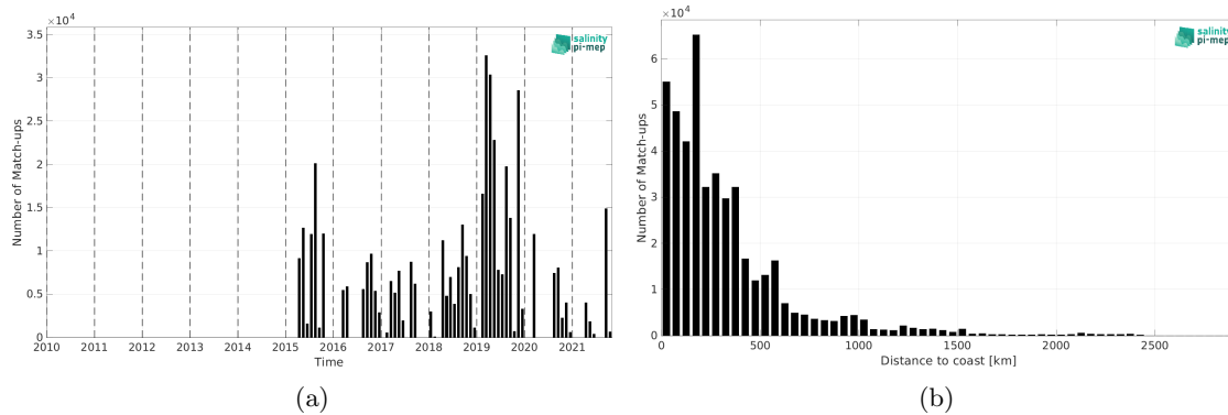
Figure 2: Number of match-ups between TSG (GOSUD-Research-vessel) and SMAP SSS L3 v5.3 - Monthly (RSS) SSS as a function of time (a) and as function of the distance to coast (b) over the Tropical Pacific Ocean Pi-MEP region and for the full satellite product period.
