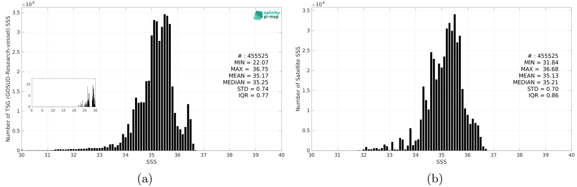
Figure 3: Histograms of SSS from TSG (GOSUD-Research-vessel) (a) and SMAP SSS L3 v5.3 - Monthly (RSS) (b) considering all match-up pairs per bins of 0.1 over the Tropical Pacific Ocean Pi-MEP region and for the full satellite product period.
