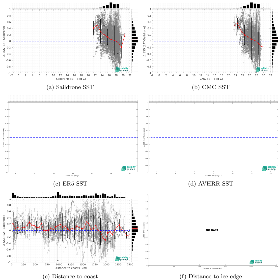
Figure 13: \Delta SSS (Satellite - Saldrone) sorted as function of Saldrone SST values (a), CMC SST (b), ERA5 SST (c), AVHRR SST (d), distance to coast (e) and distance to ice edge (f). In all plots the median and Std of \Delta SSS for each bin is indicated by the red curves and black vertical thick bars ( \pm 1 Std). Links to similar figures sorted as function of Sea ice fraction and in situ measurement depth .
