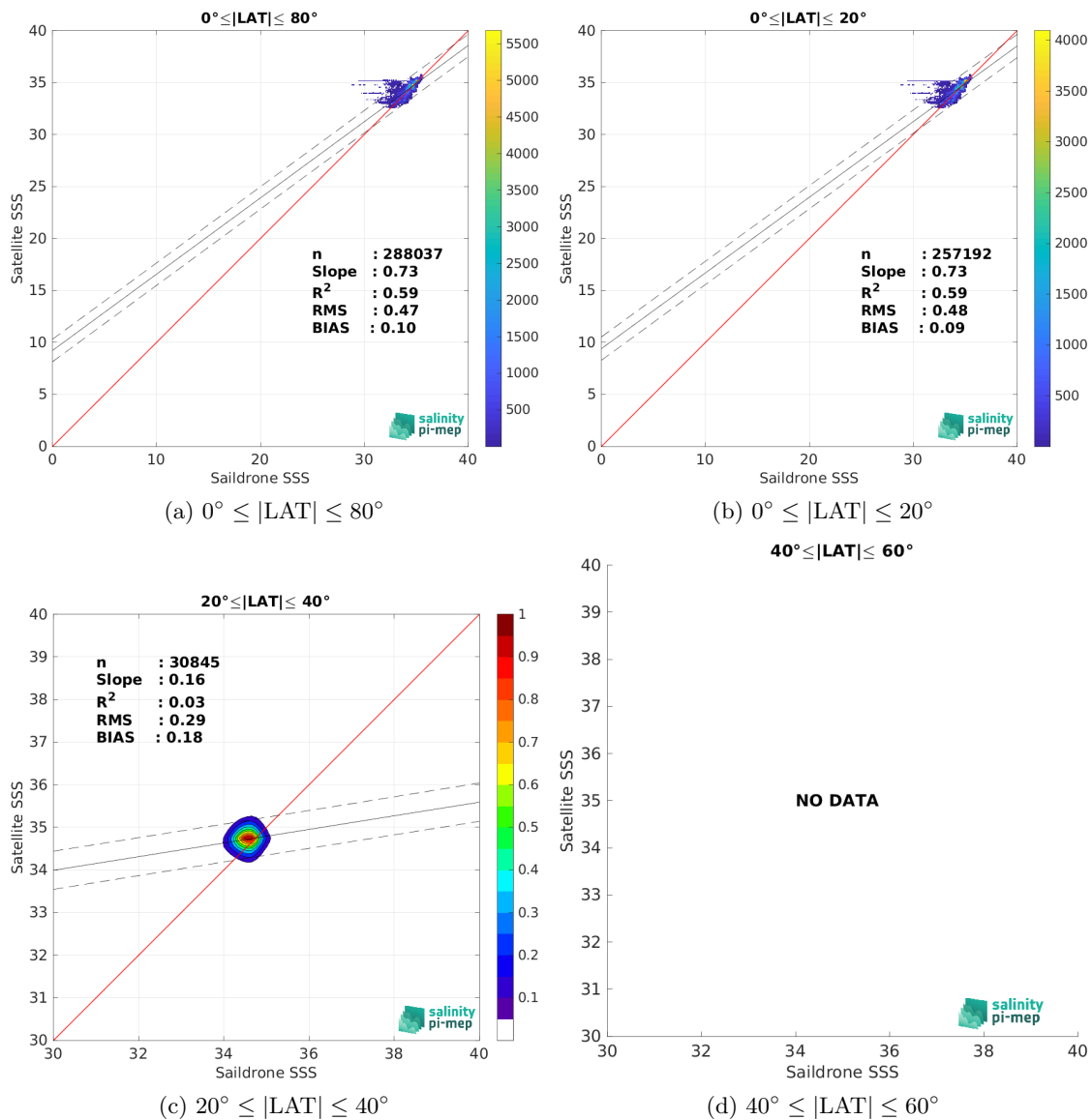
Figure 10: Contour maps of the concentration of SMAP SSS L3 v5.3 - Monthly (RSS) SSS (y-axis) versus Sairdrone SSS (x-axis) at match-up pairs for different latitude bands. For each plot, the red line shows x=y . The black thin and dashed lines indicate a linear fit through the data cloud and the \pm 95\% confidence levels, respectively. The number match-up pairs n , the slope and R^2 coefficient of the linear fit, the root mean square (RMS) and the mean bias between satellite and in situ data are indicated for each latitude band in each plots.
