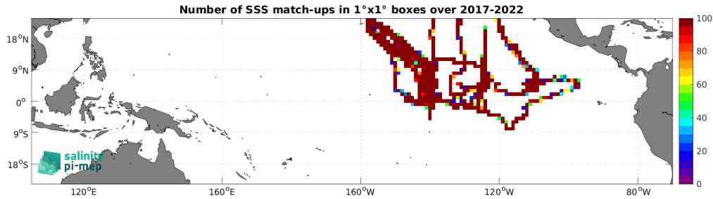
Figure 5: Number of SSS match-ups between Saildrone SSS and the SMAP SSS L3 v5.3 - Monthly (RSS) SSS product for the Tropical Pacific Ocean Pi-MEP region over 1^\circ \times 1^\circ boxes and for the full satellite product period.
