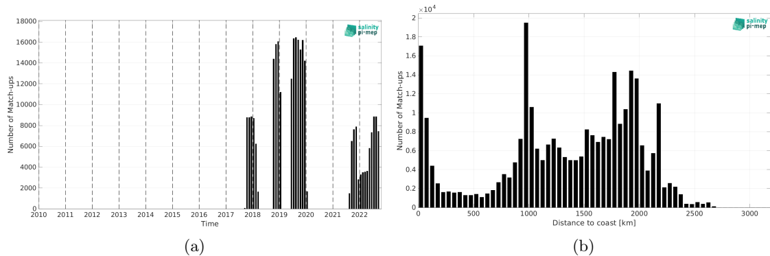
Figure 2: Number of match-ups between Saildrone and SMAP SSS L3 v5.3 - Monthly (RSS) SSS as a function of time (a) and as function of the distance to coast (b) over the Tropical Pacific Ocean Pi-MEP region and for the full satellite product period.
