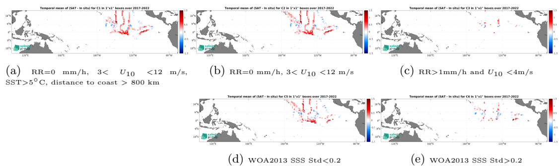
Figure 14: Temporal mean gridded over spatial boxes of size 1^\circ \times 1^\circ of \Delta SSS (SMAP SSS L3 v5.3 - Monthly (RSS) - Saildrone) for 5 different subdatasets corresponding to:RR=0 mm/h, 3 < U_{10} < 12 m/s, SST > 5^\circ\text{C} , distance to coast > 800 km (a), RR=0 mm/h, 3 < U_{10} < 12 m/s (b), RR > 1 mm/h and U_{10} < 4 m/s (c), WOA2013 SSS Std < 0.2 (d), WOA2013 SSS Std > 0.2 (e).
