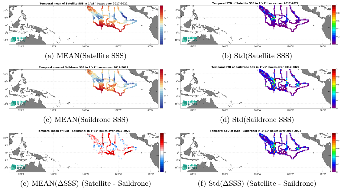
Figure 7: Temporal mean (left) and Std (right) of SSS from SMAP SSS L3 v5.3 - Monthly (RSS) (top), Saildrone (middle), and of \Delta SSS (Satellite - Saildrone). Only match-up pairs are used to generate these maps.
