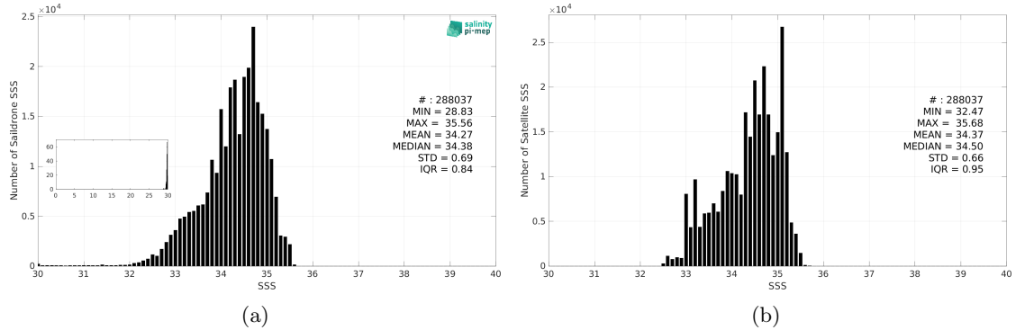
Figure 3: Histograms of SSS from Saildrone (a) and SMAP SSS L3 v5.3 - Monthly (RSS) (b) considering all match-up pairs per bins of 0.1 over the Tropical Pacific Ocean Pi-MEP region and for the full satellite product period.
