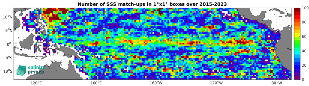
Figure 5: Number of SSS match-ups between Argo SSS and the SMAP SSS L3 v5.3 - Monthly (RSS) SSS product for the Tropical Pacific Ocean Pi-MEP region over 1^\circ \times 1^\circ boxes and for the full satellite product period.
