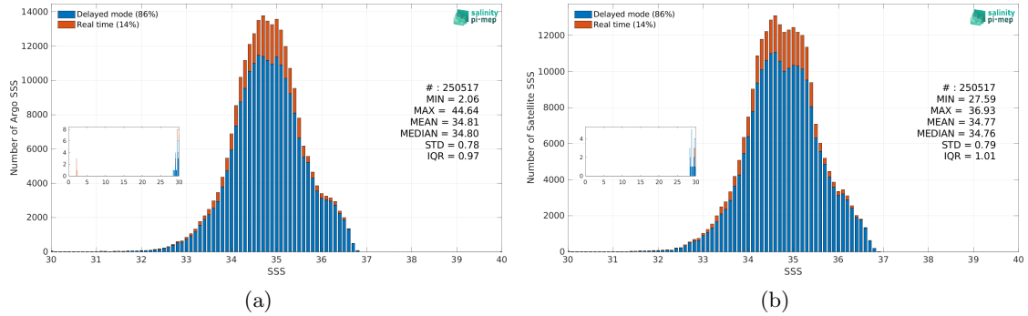
Figure 3: Histograms of SSS from Argo (a) and SMAP SSS L3 v5.3 - Monthly (RSS) (b) considering all match-up pairs per bins of 0.1 over the Tropical Pacific Ocean Pi-MEP region and for the full satellite product period.
