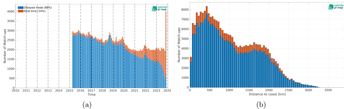
Figure 2: Number of match-ups between Argo and SMAP SSS L3 v5.3 - Monthly (RSS) SSS as a function of time (a) and as function of the distance to coast (b) over the Tropical Pacific Ocean Pi-MEP region and for the full satellite product period.
