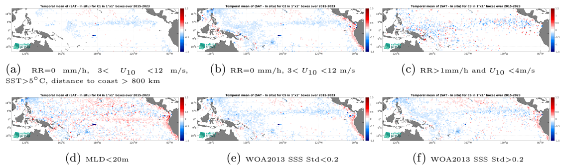
Figure 14: Temporal mean gridded over spatial boxes of size 1^\circ \times 1^\circ of \Delta SSS (SMAP SSS L3 v5.3 - Monthly (RSS) - Argo) for 6 different subdatasets corresponding to:RR=0 mm/h, 3 < U_{10} < 12 m/s, SST >5^\circ C, distance to coast > 800 km (a), RR=0 mm/h, 3 < U_{10} < 12 m/s (b), RR >1 mm/h and U_{10} < 4 m/s (c),MLD <20 m (d),WOA2013 SSS Std <0.2 (e),WOA2013 SSS Std >0.2 (f).
