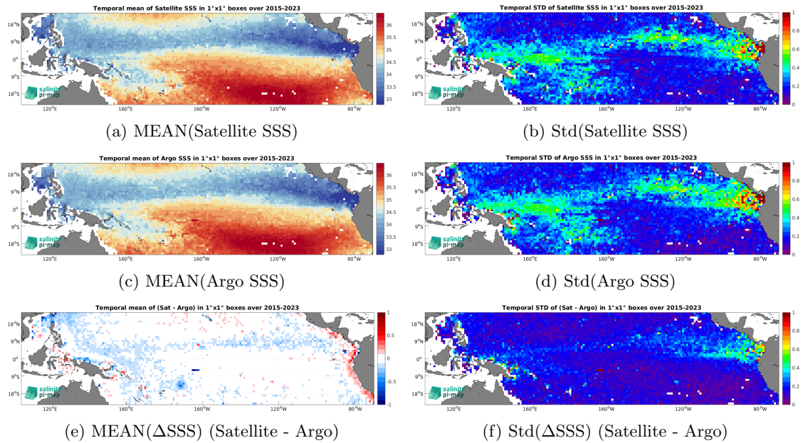
Figure 7: Temporal mean (left) and Std (right) of SSS from SMAP SSS L3 v5.3 - Monthly (RSS) (top), Argo (middle), and of \Delta SSS (Satellite - Argo). Only match-up pairs are used to generate these maps.
