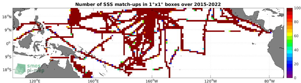
Figure 4: Number of SSS match-ups between TSG (SAMOS) SSS and the SMAP SSS L3 v5 - 8-Day running (RSS) SSS product for the Tropical Pacific Ocean Pi-MEP region over 1^\circ \times 1^\circ boxes and for the full satellite product period.
