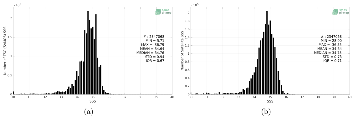
Figure 2: Histograms of SSS from TSG (SAMOS) (a) and SMAP SSS L3 v5 - 8-Day running (RSS) (b) considering all match-up pairs per bins of 0.1 over the Tropical Pacific Ocean Pi-MEP region and for the full satellite product period.
