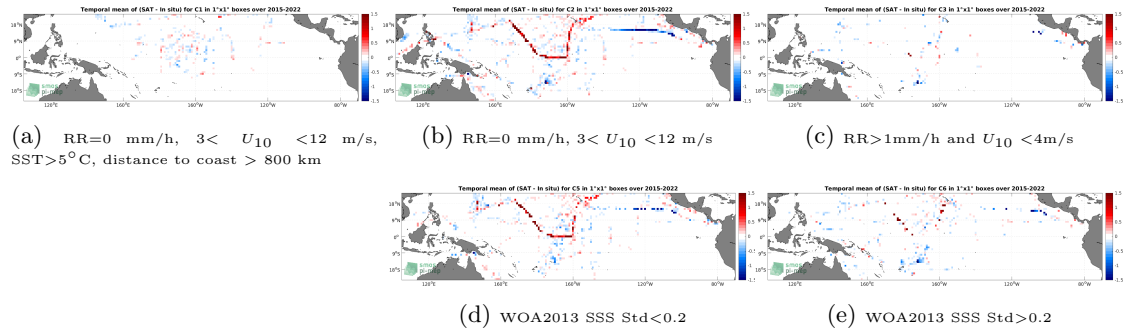
Figure 12: Temporal mean gridded over spatial boxes of size 1^\circ \times 1^\circ of \Delta SSS (SMAP SSS L3 v5 - 8-Day running (RSS) - TSG (SAMOS)) for 5 different subdatasets corresponding to:RR=0 mm/h, 3 < U_{10} < 12 m/s, SST > 5^\circ\text{C} , distance to coast > 800 km (a), RR=0 mm/h, 3 < U_{10} < 12 m/s (b), RR > 1 mm/h and U_{10} < 4 m/s (c), WOA2013 SSS Std < 0.2 (d), WOA2013 SSS Std > 0.2 (e).
