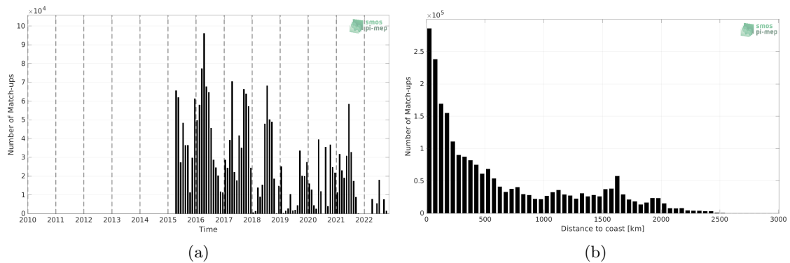
Figure 1: Number of match-ups between TSG (SAMOS) and SMAP SSS L3 v5 - 8-Day running (RSS) SSS as a function of time (a) and as function of the distance to coast (b) over the Tropical Pacific Ocean Pi-MEP region and for the full satellite product period.
