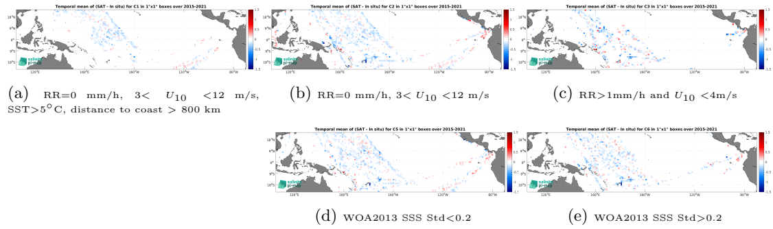
Figure 12: Temporal mean gridded over spatial boxes of size 1^\circ \times 1^\circ of \Delta\text{SSS} (SMAP SSS L3 v5 - 8-Day running (RSS) - TSG (LEGOS-DM)) for 5 different subdatasets corresponding to: \text{RR}=0 mm/h, 3 < U_{10} < 12 m/s, \text{SST} > 5^\circ\text{C} , distance to coast > 800 km (a), \text{RR}=0 mm/h, 3 < U_{10} < 12 m/s (b), \text{RR} > 1\text{mm/h} and U_{10} < 4\text{m/s} (c), WOA2013 SSS Std < 0.2 (d), WOA2013 SSS Std > 0.2 (e).
