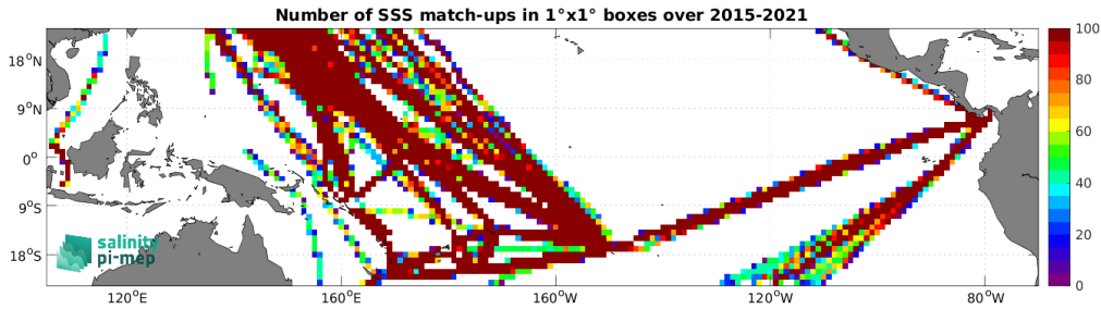
Figure 4: Number of SSS match-ups between TSG (LEGOS-DM) SSS and the SMAP SSS L3 v5 - 8-Day running (RSS) SSS product for the Tropical Pacific Ocean Pi-MEP region over 1^\circ \times 1^\circ boxes and for the full satellite product period.
