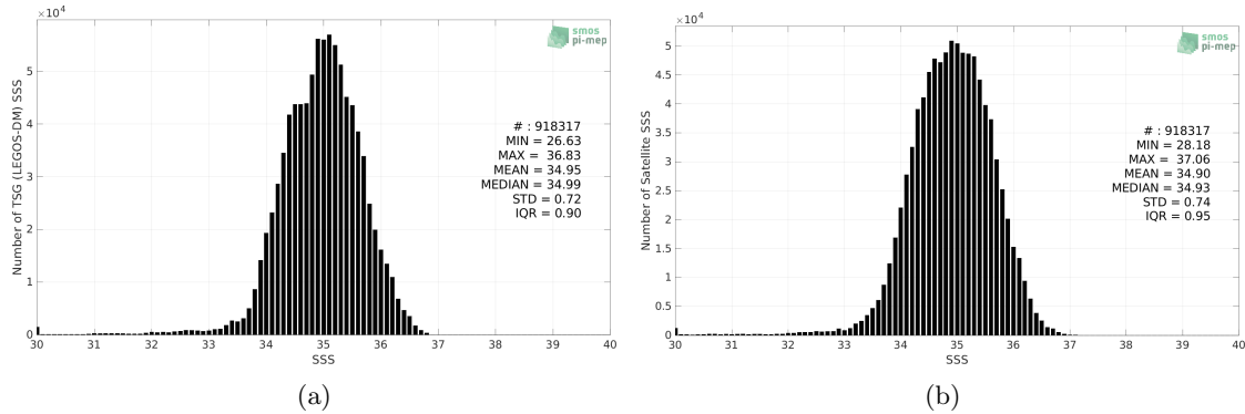
Figure 2: Histograms of SSS from TSG (LEGOS-DM) (a) and SMAP SSS L3 v5 - 8-Day running (RSS) (b) considering all match-up pairs per bins of 0.1 over the Tropical Pacific Ocean Pi-MEP region and for the full satellite product period.
