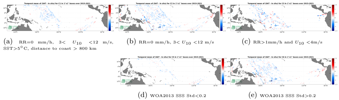
Figure 12: Temporal mean gridded over spatial boxes of size 1^\circ \times 1^\circ of \Delta SSS (SMAP SSS L3 v5 - 8-Day running (RSS) - TSG (LEGOS-DM)) for 5 different subdatasets corresponding to:RR=0 mm/h, 3 < U_{10} < 12 m/s, SST > 5^\circ\text{C} , distance to coast > 800 km (a), RR=0 mm/h, 3 < U_{10} < 12 m/s (b), RR > 1 mm/h and U_{10} < 4 m/s (c), WOA2013 SSS Std < 0.2 (d), WOA2013 SSS Std > 0.2 (e).
