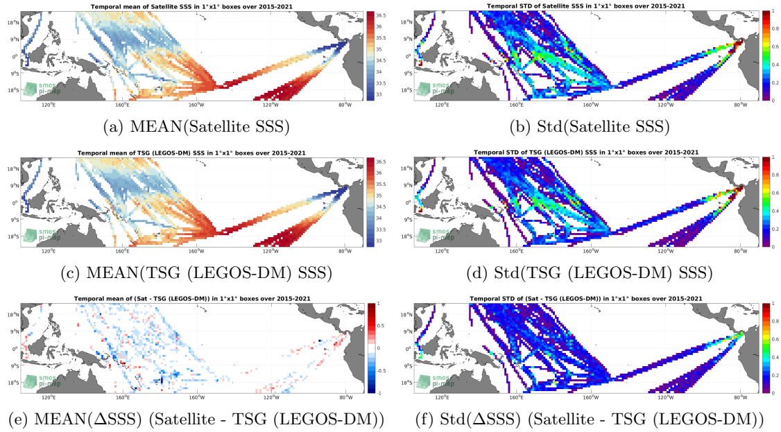
Figure 6: Temporal mean (left) and Std (right) of SSS from SMAP SSS L3 v5 - 8-Day running (RSS) (top), TSG (LEGOS-DM) (middle), and of \Delta SSS (Satellite - TSG (LEGOS-DM)). Only match-up pairs are used to generate these maps.
