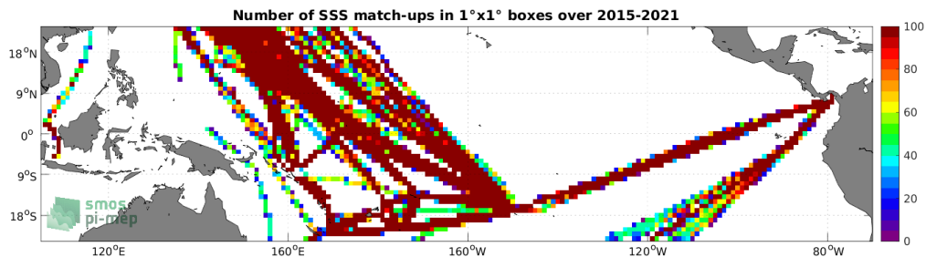
Figure 4: Number of SSS match-ups between TSG (LEGOS-DM) SSS and the SMAP SSS L3 v5 - 8-Day running (RSS) SSS product for the Tropical Pacific Ocean Pi-MEP region over 1^\circ \times 1^\circ boxes and for the full satellite product period.
