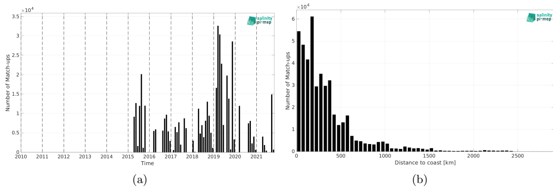
Figure 1: Number of match-ups between TSG (GOSUD-Research-vessel) and SMAP SSS L3 v5 - 8-Day running (RSS) SSS as a function of time (a) and as function of the distance to coast (b) over the Tropical Pacific Ocean Pi-MEP region and for the full satellite product period.
