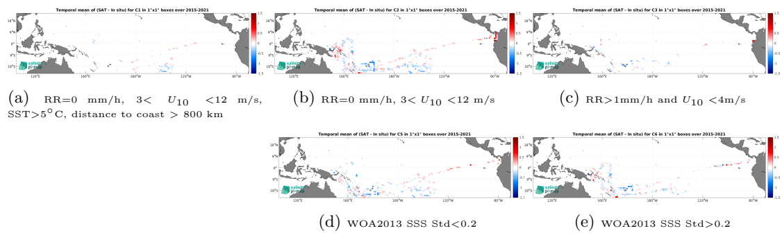
Figure 12: Temporal mean gridded over spatial boxes of size 1^\circ \times 1^\circ of \Delta SSS (SMAP SSS L3 v5 - 8-Day running (RSS) - TSG (GOSUD-Research-vessel)) for 5 different subdatasets corresponding to:RR=0 mm/h, 3 < U_{10} < 12 m/s, SST >5^\circ C, distance to coast > 800 km (a), RR=0 mm/h, 3 < U_{10} < 12 m/s (b), RR >1 mm/h and U_{10} < 4 m/s (c), WOA2013 SSS Std <0.2 (d), WOA2013 SSS Std >0.2 (e).
