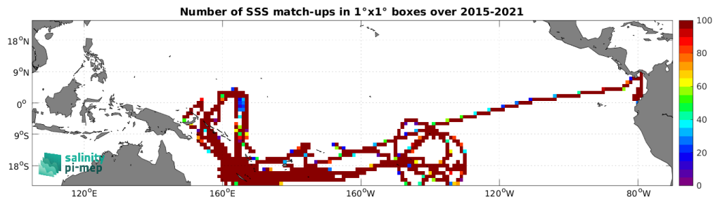
Figure 4: Number of SSS match-ups between TSG (GOSUD-Research-vessel) SSS and the SMAP SSS L3 v5 - 8-Day running (RSS) SSS product for the Tropical Pacific Ocean Pi-MEP region over 1^\circ \times 1^\circ boxes and for the full satellite product period.
