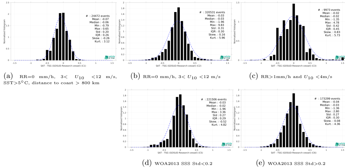
Figure 13: Normalized histogram of \Delta\text{SSS} (SMAP SSS L3 v5 - 8-Day running (RSS) - TSG (GOSUD-Research-vessel)) for 5 different subdatasets corresponding to: RR=0 mm/h, 3 < U_{10} < 12 m/s, SST > 5^\circ\text{C} , distance to coast > 800 km (a), RR=0 mm/h, 3 < U_{10} < 12 m/s (b), RR > 1 mm/h and U_{10} < 4 m/s (c), WOA2013 SSS Std < 0.2 (d), WOA2013 SSS Std > 0.2 (e).
