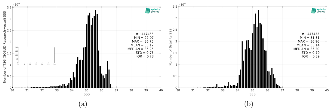
Figure 2: Histograms of SSS from TSG (GOSUD-Research-vessel) (a) and SMAP SSS L3 v5 - 8-Day running (RSS) (b) considering all match-up pairs per bins of 0.1 over the Tropical Pacific Ocean Pi-MEP region and for the full satellite product period.
