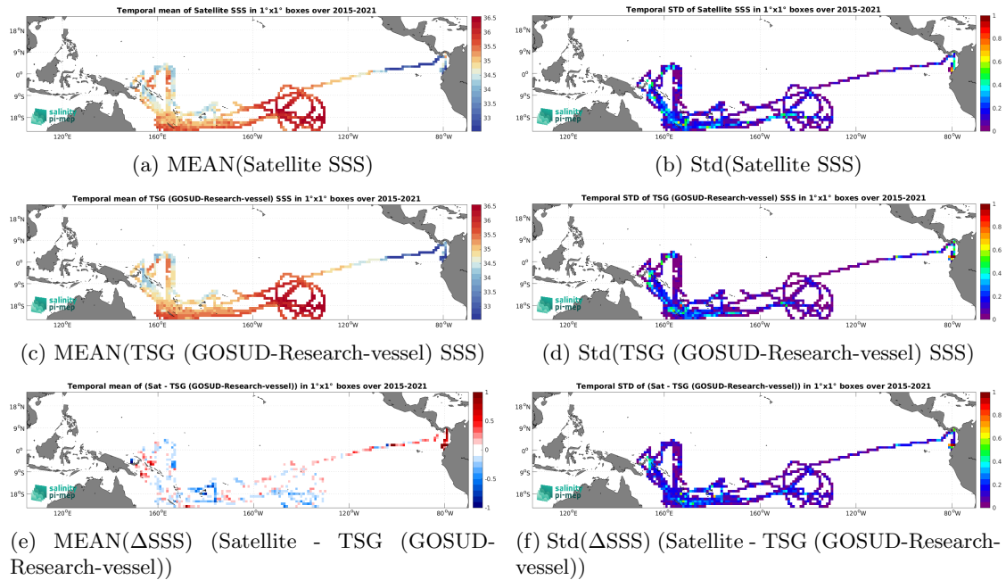
Figure 6: Temporal mean (left) and Std (right) of SSS from SMAP SSS L3 v5 - 8-Day running (RSS) (top), TSG (GOSUD-Research-vessel) (middle), and of \Delta SSS (Satellite - TSG (GOSUD-Research-vessel)). Only match-up pairs are used to generate these maps.
