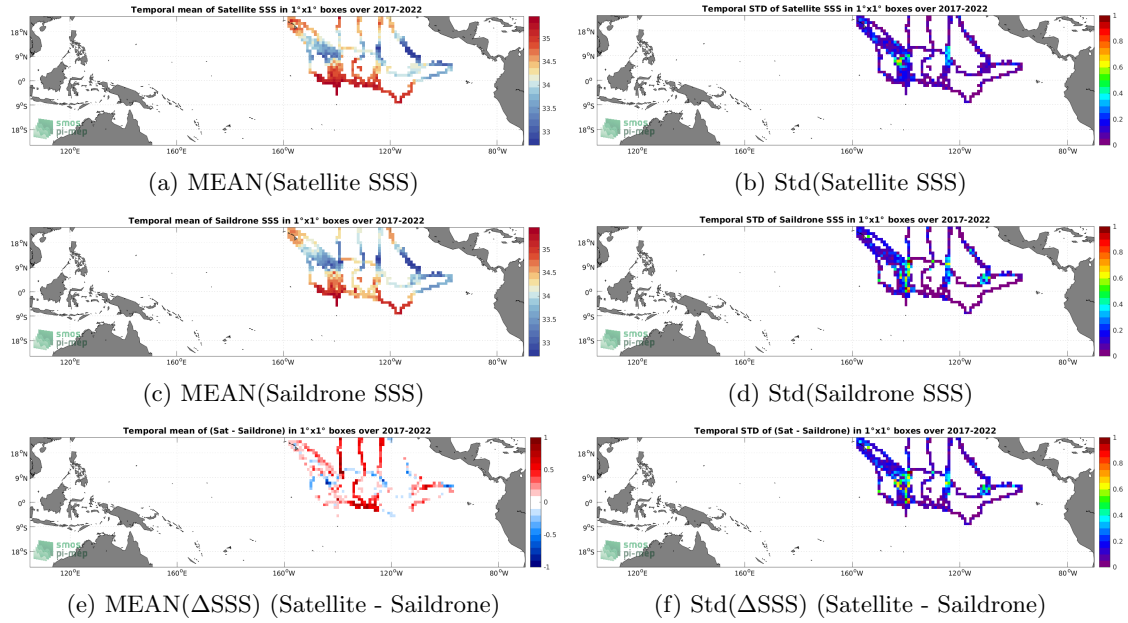
Figure 6: Temporal mean (left) and Std (right) of SSS from SMAP SSS L3 v5 - 8-Day running (RSS) (top), Saildrone (middle), and of \Delta SSS (Satellite - Saildrone). Only match-up pairs are used to generate these maps.
