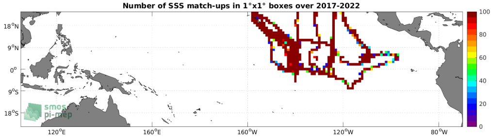
Figure 4: Number of SSS match-ups between Saildrone SSS and the SMAP SSS L3 v5 - 8-Day running (RSS) SSS product for the Tropical Pacific Ocean Pi-MEP region over 1^\circ \times 1^\circ boxes and for the full satellite product period.
