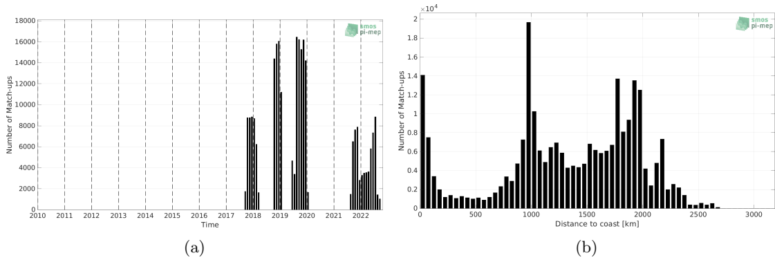
Figure 1: Number of match-ups between Saildrone and SMAP SSS L3 v5 - 8-Day running (RSS) SSS as a function of time (a) and as function of the distance to coast (b) over the Tropical Pacific Ocean Pi-MEP region and for the full satellite product period.
