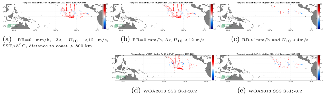
Figure 12: Temporal mean gridded over spatial boxes of size 1^\circ \times 1^\circ of \Delta SSS (SMAP SSS L3 v5 - 8-Day running (RSS) - Saildrone) for 5 different subdatasets corresponding to:RR=0 mm/h, 3 < U_{10} < 12 m/s, SST > 5^\circ C , distance to coast > 800 km (a), RR=0 mm/h, 3 < U_{10} < 12 m/s (b), RR>1mm/h and U_{10} < 4 m/s (c), WOA2013 SSS Std<0.2 (d), WOA2013 SSS Std>0.2 (e).
