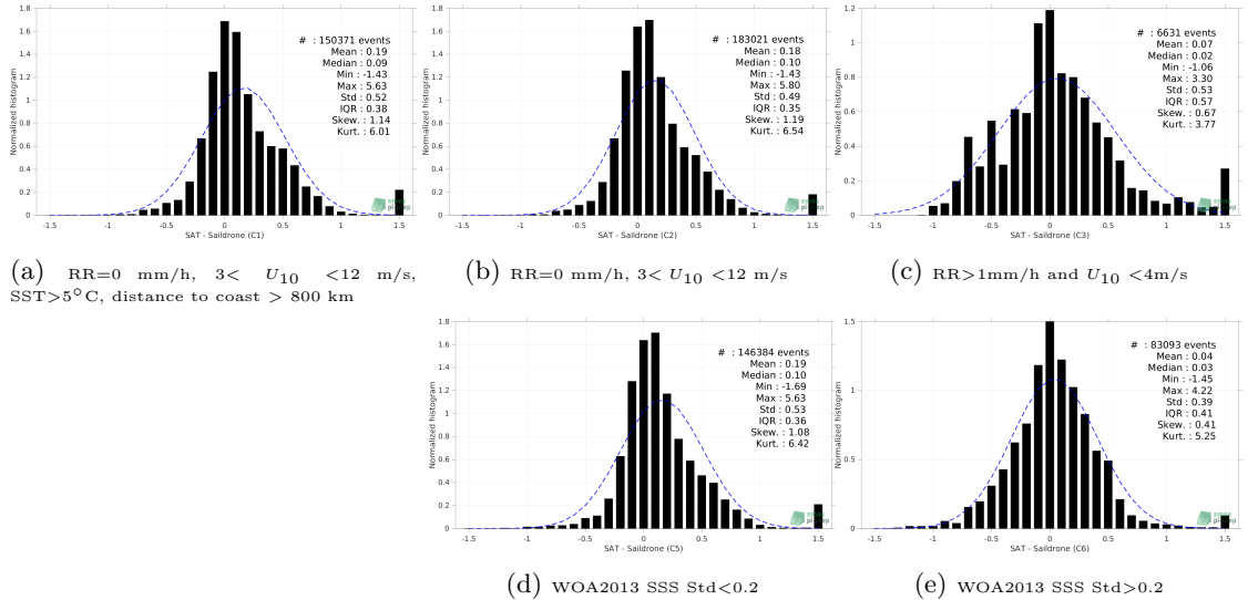
Figure 13: Normalized histogram of \Delta SSS (SMAP SSS L3 v5 - 8-Day running (RSS) - Saildrone) for 5 different subdatasets corresponding to: RR=0 mm/h, 3 < U_{10} < 12 m/s, SST > 5^\circ C , distance to coast > 800 km (a), RR=0 mm/h, 3 < U_{10} < 12 m/s (b), RR>1mm/h and U_{10} < 4 m/s (c), WOA2013 SSS Std<0.2 (d), WOA2013 SSS Std>0.2 (e).
