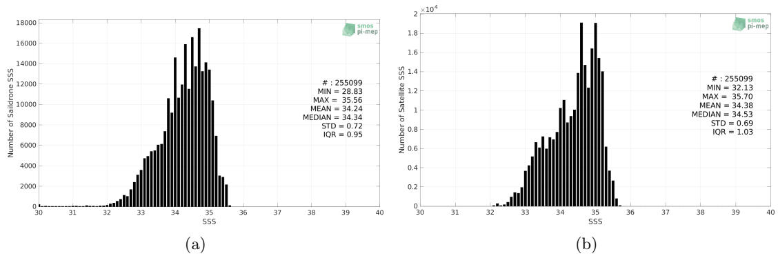
Figure 2: Histograms of SSS from Saildrone (a) and SMAP SSS L3 v5 - 8-Day running (RSS) (b) considering all match-up pairs per bins of 0.1 over the Tropical Pacific Ocean Pi-MEP region and for the full satellite product period.
