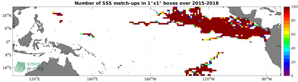
Figure 3: Number of SSS match-ups between Surface drifters SSS and the SMAP SSS L3 v5 - 8-Day running (RSS) SSS product for the Tropical Pacific Ocean Pi-MEP region over 1^\circ \times 1^\circ boxes and for the full satellite product period.
