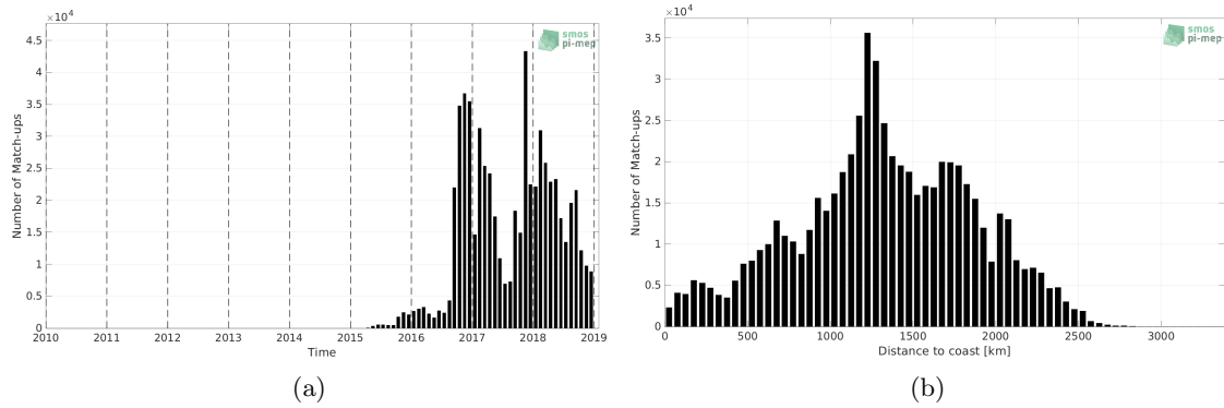
Figure 1: Number of match-ups between Surface drifters and SMAP SSS L3 v5 - 8-Day running (RSS) SSS as a function of time (a) and as function of the distance to coast (b) over the Tropical Pacific Ocean Pi-MEP region and for the full satellite product period.
