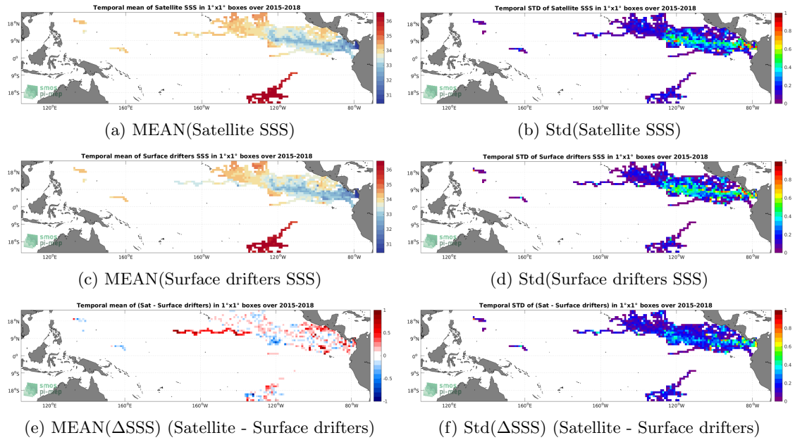
Figure 5: Temporal mean (left) and Std (right) of SSS from SMAP SSS L3 v5 - 8-Day running (RSS) (top), Surface drifters (middle), and of \Delta SSS (Satellite - Surface drifters). Only match-up pairs are used to generate these maps.
