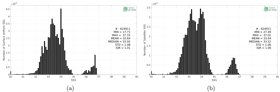
Figure 2: Histograms of SSS from Surface drifters (a) and SMAP SSS L3 v5 - 8-Day running (RSS) (b) considering all match-up pairs per bins of 0.1 over the Tropical Pacific Ocean Pi-MEP region and for the full satellite product period.
