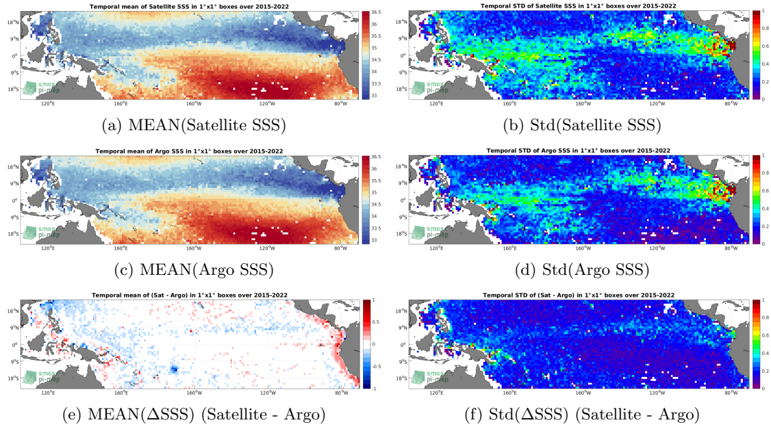
Figure 6: Temporal mean (left) and Std (right) of SSS from SMAP SSS L3 v5 - 8-Day running (RSS) (top), Argo (middle), and of \Delta SSS (Satellite - Argo). Only match-up pairs are used to generate these maps.
