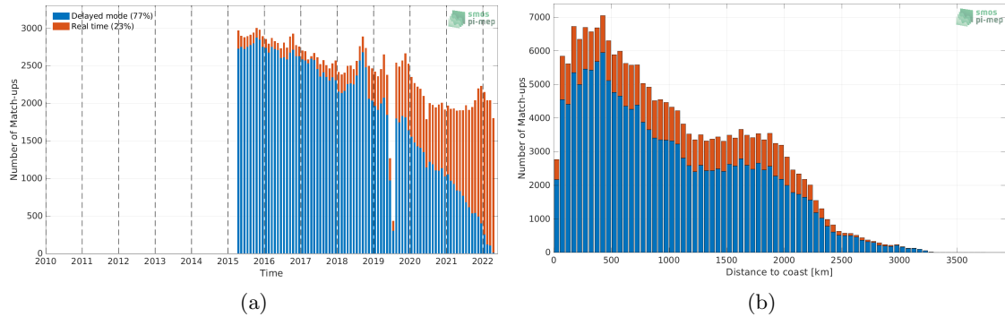
Figure 1: Number of match-ups between Argo and SMAP SSS L3 v5 - 8-Day running (RSS) SSS as a function of time (a) and as function of the distance to coast (b) over the Tropical Pacific Ocean Pi-MEP region and for the full satellite product period.
