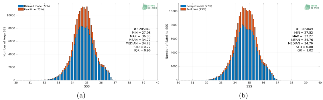
Figure 2: Histograms of SSS from Argo (a) and SMAP SSS L3 v5 - 8-Day running (RSS) (b) considering all match-up pairs per bins of 0.1 over the Tropical Pacific Ocean Pi-MEP region and for the full satellite product period.
