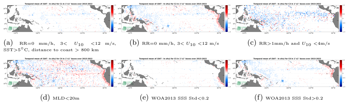
Figure 12: Temporal mean gridded over spatial boxes of size 1^\circ \times 1^\circ of \Delta SSS (SMAP SSS L3 v5 - 8-Day running (RSS) - Argo) for 6 different subdatasets corresponding to:RR=0 mm/h, 3 < U_{10} < 12 m/s, SST >5^\circ C, distance to coast > 800 km (a), RR=0 mm/h, 3 < U_{10} < 12 m/s (b), RR >1 mm/h and U_{10} < 4 m/s (c),MLD <20 m (d),WOA2013 SSS Std <0.2 (e),WOA2013 SSS Std >0.2 (f).
