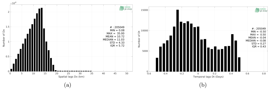
Figure 5: Histograms of the spatial (a) and temporal (b) lags between the location/time of the Argo measurement and the date of the corresponding SMAP SSS L3 v5 - 8-Day running (RSS) SSS pixel.
