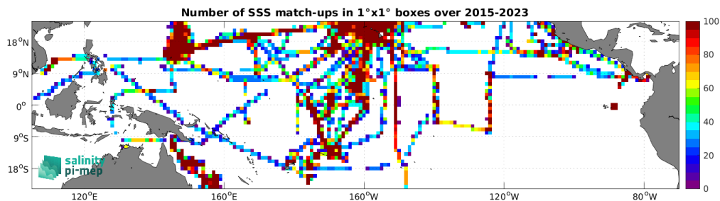
Figure 4: Number of SSS match-ups between TSG (SAMOS) SSS and the SMAP SSS L3 v5 - Monthly (RSS) SSS product for the Tropical Pacific Ocean Pi-MEP region over 1^\circ \times 1^\circ boxes and for the full satellite product period.
