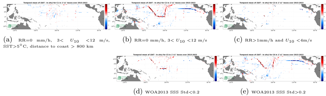
Figure 12: Temporal mean gridded over spatial boxes of size 1^\circ \times 1^\circ of \Delta\text{SSS} (SMAP SSS L3 v5 - Monthly (RSS) - TSG (SAMOS)) for 5 different subdatasets corresponding to: RR=0 mm/h, 3 < U_{10} < 12 m/s, SST >5^\circ\text{C} , distance to coast > 800 km (a), RR=0 mm/h, 3 < U_{10} < 12 m/s (b), RR >1 mm/h and U_{10} < 4 m/s (c), WOA2013 SSS Std <0.2 (d), WOA2013 SSS Std >0.2 (e).
