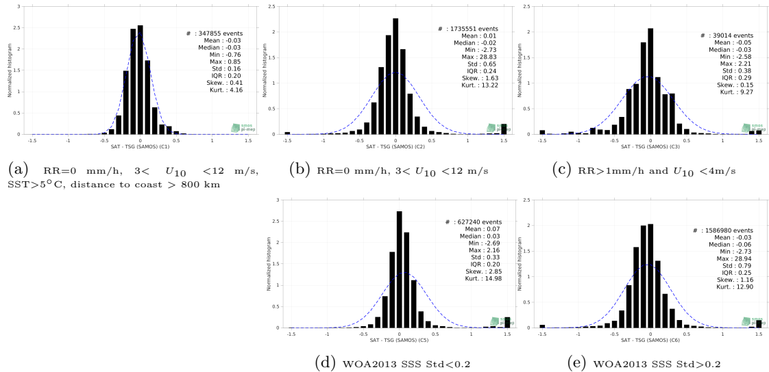
Figure 13: Normalized histogram of \Delta\text{SSS} (SMAP SSS L3 v5 - Monthly (RSS) - TSG (SAMOS)) for 5 different subdatasets corresponding to: RR=0 mm/h, 3 < U_{10} < 12 m/s, SST >5^\circ\text{C} , distance to coast > 800 km (a), RR=0 mm/h, 3 < U_{10} < 12 m/s (b), RR >1 mm/h and U_{10} < 4 m/s (c), WOA2013 SSS Std <0.2 (d), WOA2013 SSS Std >0.2 (e).
