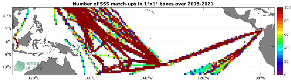
Figure 4: Number of SSS match-ups between TSG (LEGOS-DM) SSS and the SMAP SSS L3 v5 - Monthly (RSS) SSS product for the Tropical Pacific Ocean Pi-MEP region over 1^\circ \times 1^\circ boxes and for the full satellite product period.
