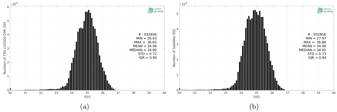
Figure 2: Histograms of SSS from TSG (LEGOS-DM) (a) and SMAP SSS L3 v5 - Monthly (RSS) (b) considering all match-up pairs per bins of 0.1 over the Tropical Pacific Ocean Pi-MEP region and for the full satellite product period.
