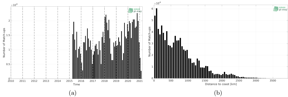
Figure 1: Number of match-ups between TSG (LEGOS-DM) and SMAP SSS L3 v5 - Monthly (RSS) SSS as a function of time (a) and as function of the distance to coast (b) over the Tropical Pacific Ocean Pi-MEP region and for the full satellite product period.
