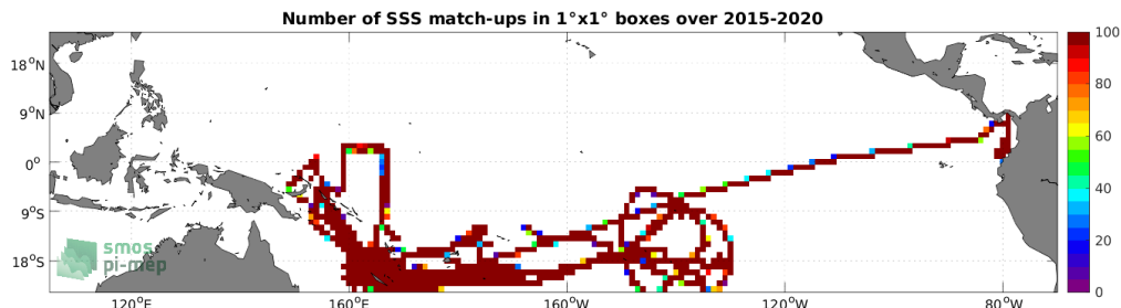
Figure 4: Number of SSS match-ups between TSG (GOSUD-Research-vessel) SSS and the SMAP SSS L3 v5 - Monthly (RSS) SSS product for the Tropical Pacific Ocean Pi-MEP region over 1^\circ \times 1^\circ boxes and for the full satellite product period.
