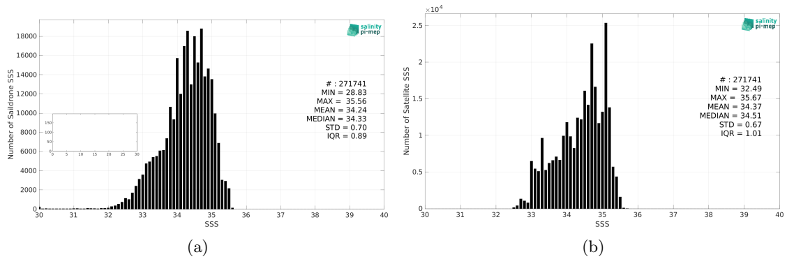
Figure 2: Histograms of SSS from Saildrone (a) and SMAP SSS L3 v5 - Monthly (RSS) (b) considering all match-up pairs per bins of 0.1 over the Tropical Pacific Ocean Pi-MEP region and for the full satellite product period.
