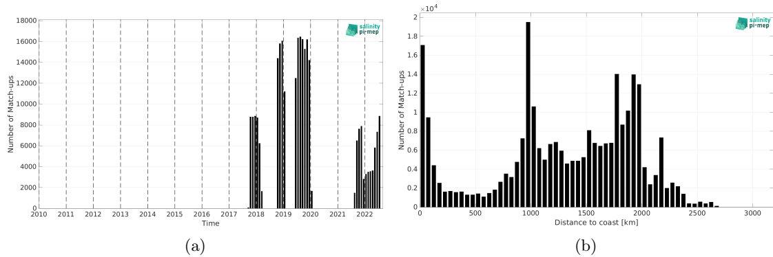
Figure 1: Number of match-ups between Saildrone and SMAP SSS L3 v5 - Monthly (RSS) SSS as a function of time (a) and as function of the distance to coast (b) over the Tropical Pacific Ocean Pi-MEP region and for the full satellite product period.
