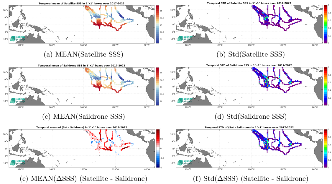
Figure 6: Temporal mean (left) and Std (right) of SSS from SMAP SSS L3 v5 - Monthly (RSS) (top), Saildrone (middle), and of \Delta SSS (Satellite - Saildrone). Only match-up pairs are used to generate these maps.
