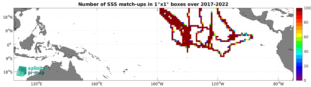
Figure 4: Number of SSS match-ups between Sairdron SSS and the SMAP SSS L3 v5 - Monthly (RSS) SSS product for the Tropical Pacific Ocean Pi-MEP region over 1^\circ \times 1^\circ boxes and for the full satellite product period.
