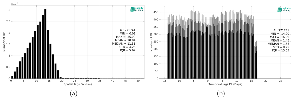
Figure 5: Histograms of the spatial (a) and temporal (b) lags between the location/time of the Sairdron measurement and the date of the corresponding SMAP SSS L3 v5 - Monthly (RSS) SSS pixel.
