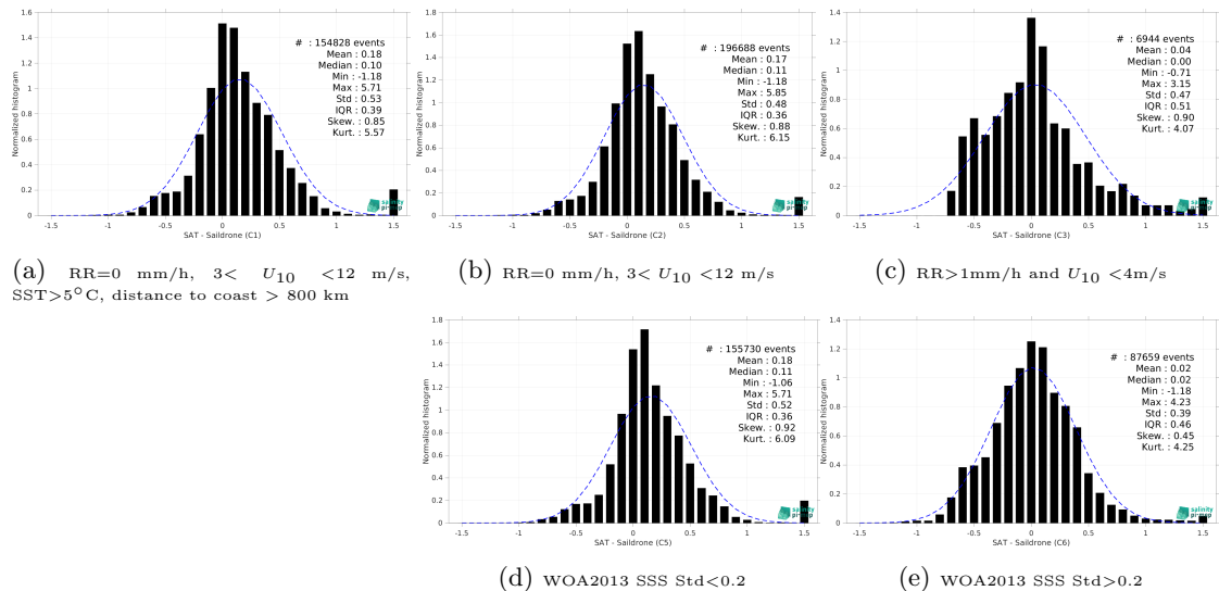
Figure 13: Normalized histogram of \Delta SSS (SMAP SSS L3 v5 - Monthly (RSS) - Saildrone) for 5 different subdatasets corresponding to: RR=0 mm/h, 3 < U_{10} < 12 m/s, SST >5^\circ\text{C} , distance to coast > 800 km (a), RR=0 mm/h, 3 < U_{10} < 12 m/s (b), RR >1 mm/h and U_{10} < 4 m/s (c), WOA2013 SSS Std <0.2 (d), WOA2013 SSS Std >0.2 (e).
