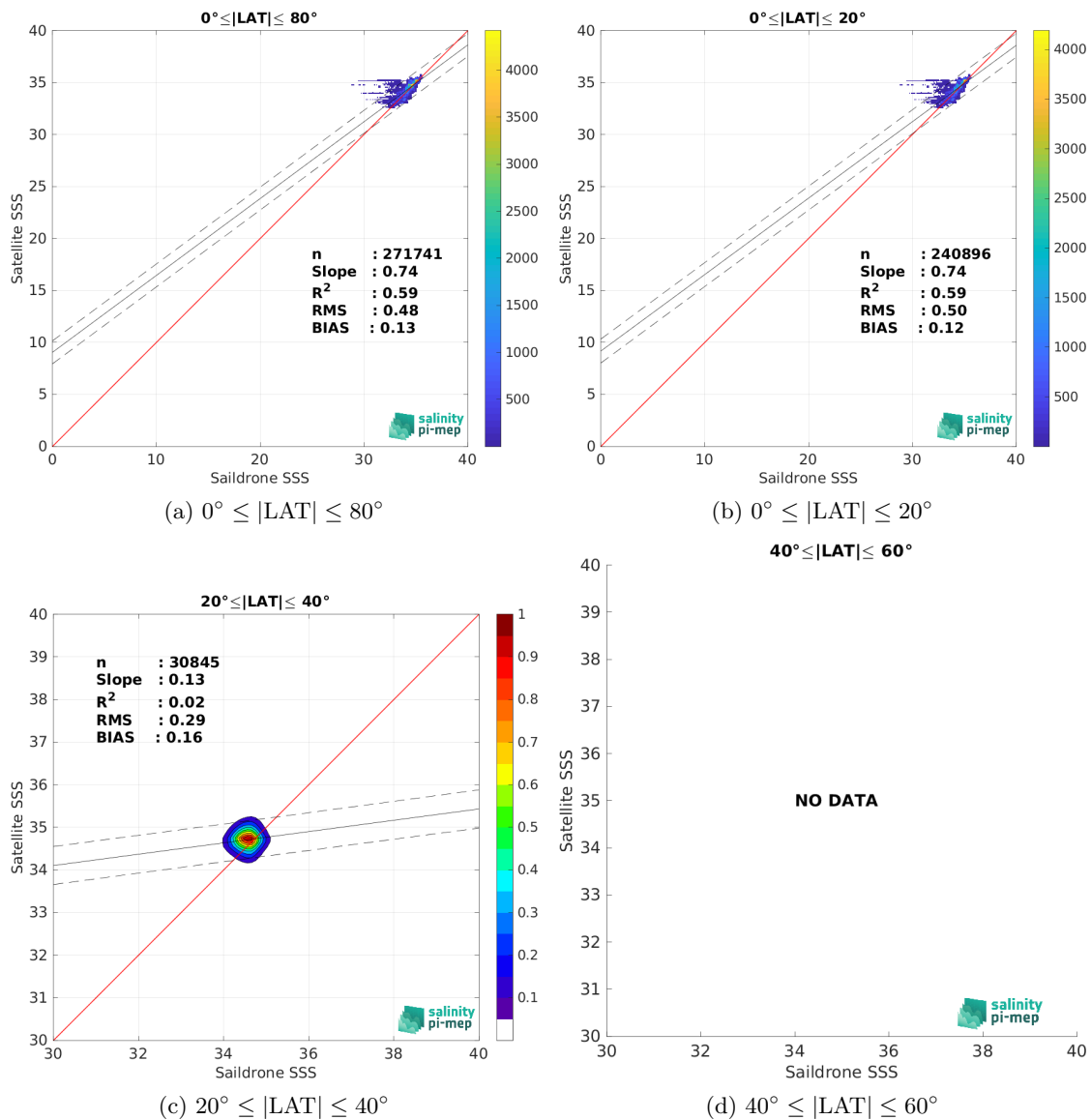
Figure 9: Contour maps of the concentration of SMAP SSS L3 v5 - Monthly (RSS) SSS (y-axis) versus Sairdrone SSS (x-axis) at match-up pairs for different latitude bands. For each plot, the red line shows x=y . The black thin and dashed lines indicate a linear fit through the data cloud and the \pm 95\% confidence levels, respectively. The number match-up pairs n , the slope and R^2 coefficient of the linear fit, the root mean square (RMS) and the mean bias between satellite and in situ data are indicated for each latitude band in each plots.
