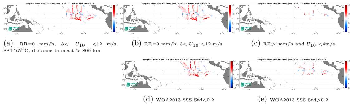
Figure 12: Temporal mean gridded over spatial boxes of size 1^\circ \times 1^\circ of \Delta SSS (SMAP SSS L3 v5 - Monthly (RSS) - Saildrone) for 5 different subdatasets corresponding to:RR=0 mm/h, 3 < U_{10} < 12 m/s, SST >5^\circ\text{C} , distance to coast > 800 km (a), RR=0 mm/h, 3 < U_{10} < 12 m/s (b), RR >1 mm/h and U_{10} < 4 m/s (c), WOA2013 SSS Std <0.2 (d), WOA2013 SSS Std >0.2 (e).
