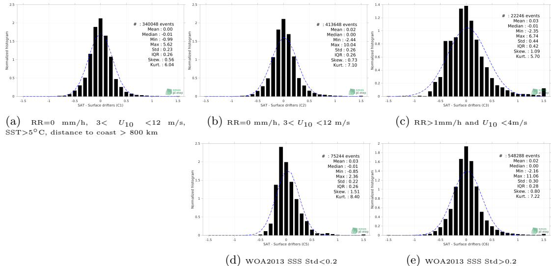
Figure 12: Normalized histogram of \Delta\text{SSS} (SMAP SSS L3 v5 - Monthly (RSS) - Surface drifters) for 5 different subdatasets corresponding to: RR=0 mm/h, 3 < U_{10} < 12 m/s, SST >5^\circ\text{C} , distance to coast > 800 km (a), RR=0 mm/h, 3 < U_{10} < 12 m/s (b), RR >1 mm/h and U_{10} < 4 m/s (c), WOA2013 SSS Std <0.2 (d), WOA2013 SSS Std >0.2 (e).
