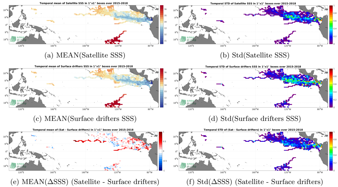
Figure 5: Temporal mean (left) and Std (right) of SSS from SMAP SSS L3 v5 - Monthly (RSS) (top), Surface drifters (middle), and of \Delta SSS (Satellite - Surface drifters). Only match-up pairs are used to generate these maps.
