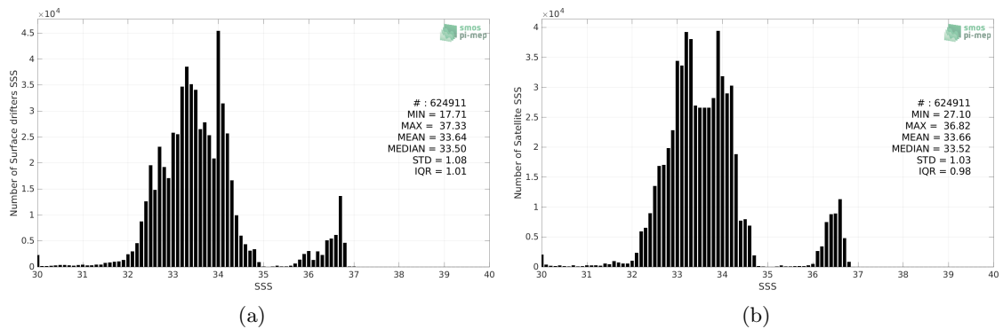
Figure 2: Histograms of SSS from Surface drifters (a) and SMAP SSS L3 v5 - Monthly (RSS) (b) considering all match-up pairs per bins of 0.1 over the Tropical Pacific Ocean Pi-MEP region and for the full satellite product period.
