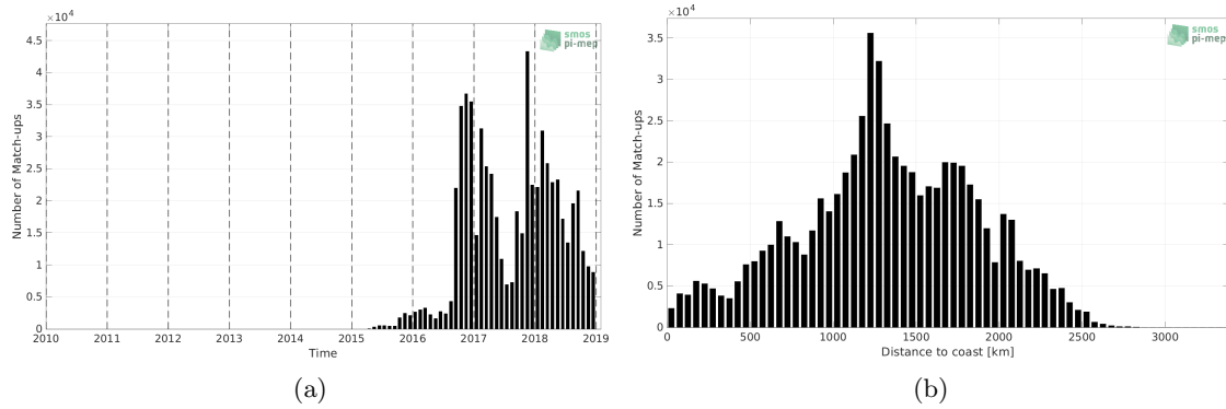
Figure 1: Number of match-ups between Surface drifters and SMAP SSS L3 v5 - Monthly (RSS) SSS as a function of time (a) and as function of the distance to coast (b) over the Tropical Pacific Ocean Pi-MEP region and for the full satellite product period.
