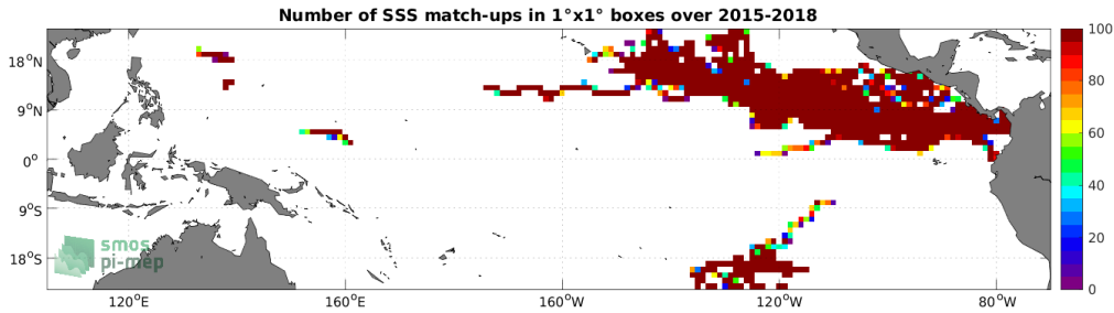
Figure 3: Number of SSS match-ups between Surface drifters SSS and the SMAP SSS L3 v5 - Monthly (RSS) SSS product for the Tropical Pacific Ocean Pi-MEP region over 1^\circ \times 1^\circ boxes and for the full satellite product period.
