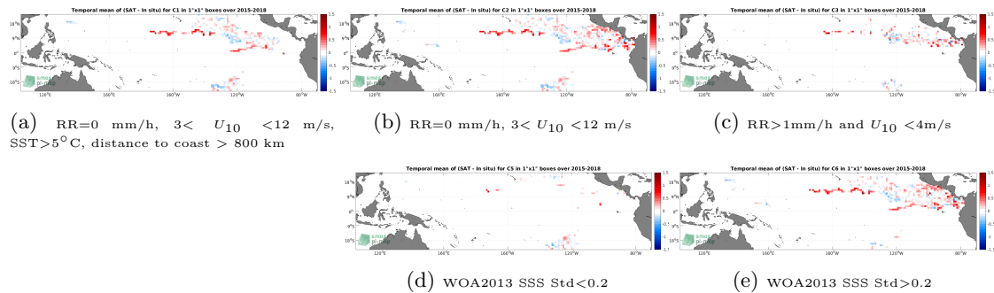
Figure 11: Temporal mean gridded over spatial boxes of size 1^\circ \times 1^\circ of \Delta\text{SSS} (SMAP SSS L3 v5 - Monthly (RSS) - Surface drifters) for 5 different subdatasets corresponding to:RR=0 mm/h, 3 < U_{10} < 12 m/s, SST >5^\circ\text{C} , distance to coast > 800 km (a), RR=0 mm/h, 3 < U_{10} < 12 m/s (b), RR >1 mm/h and U_{10} < 4 m/s (c), WOA2013 SSS Std <0.2 (d), WOA2013 SSS Std >0.2 (e).
