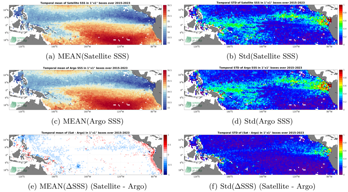
Figure 6: Temporal mean (left) and Std (right) of SSS from SMAP SSS L3 v5 - Monthly (RSS) (top), Argo (middle), and of \Delta SSS (Satellite - Argo). Only match-up pairs are used to generate these maps.
