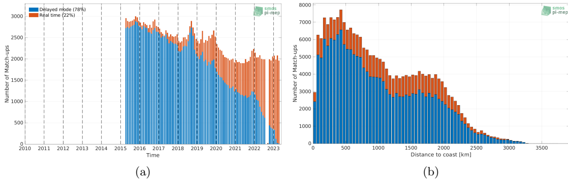
Figure 1: Number of match-ups between Argo and SMAP SSS L3 v5 - Monthly (RSS) SSS as a function of time (a) and as function of the distance to coast (b) over the Tropical Pacific Ocean Pi-MEP region and for the full satellite product period.
