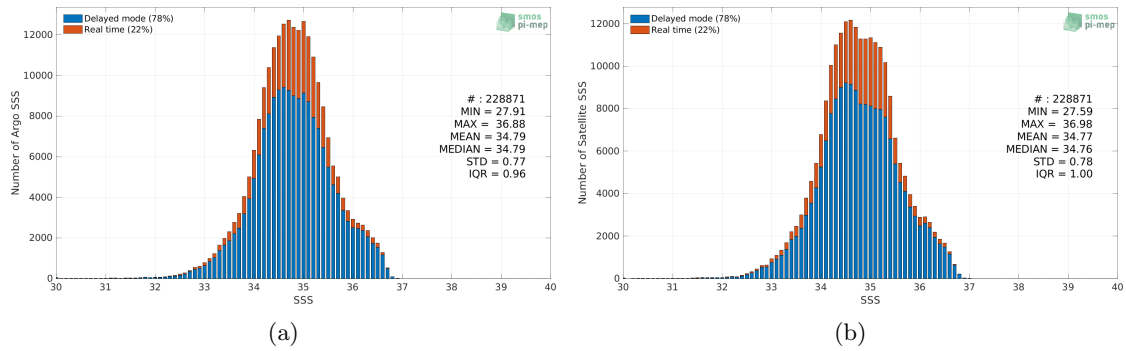
Figure 2: Histograms of SSS from Argo (a) and SMAP SSS L3 v5 - Monthly (RSS) (b) considering all match-up pairs per bins of 0.1 over the Tropical Pacific Ocean Pi-MEP region and for the full satellite product period.
