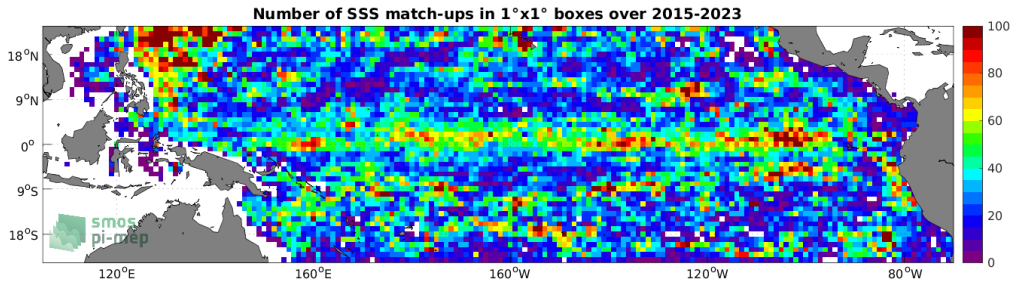
Figure 4: Number of SSS match-ups between Argo SSS and the SMAP SSS L3 v5 - Monthly (RSS) SSS product for the Tropical Pacific Ocean Pi-MEP region over 1^\circ \times 1^\circ boxes and for the full satellite product period.
