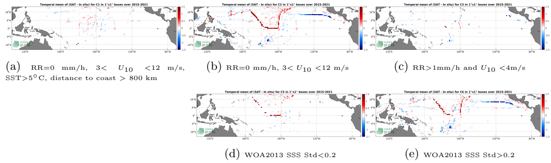
Figure 12: Temporal mean gridded over spatial boxes of size 1^\circ \times 1^\circ of \Delta SSS (SMAP SSS L3 v4 - 8-Day running (RSS) - TSG (SAMOS)) for 5 different subdatasets corresponding to: RR=0 mm/h, 3 < U_{10} < 12 m/s, SST > 5^\circ C , distance to coast > 800 km (a), RR=0 mm/h, 3 < U_{10} < 12 m/s (b), RR > 1 mm/h and U_{10} < 4 m/s (c), WOA2013 SSS Std < 0.2 (d), WOA2013 SSS Std > 0.2 (e).
