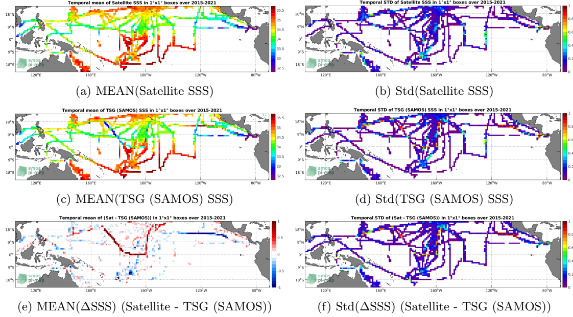
Figure 6: Temporal mean (left) and Std (right) of SSS from SMAP SSS L3 v4 - 8-Day running (RSS) (top), TSG (SAMOS) (middle), and of \Delta SSS (Satellite - TSG (SAMOS)). Only match-up pairs are used to generate these maps.
