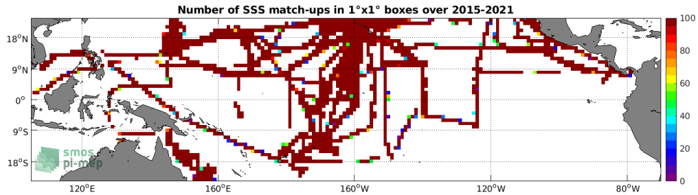
Figure 4: Number of SSS match-ups between TSG (SAMOS) SSS and the SMAP SSS L3 v4 - 8-Day running (RSS) SSS product for the Tropical Pacific Ocean Pi-MEP region over 1^\circ \times 1^\circ boxes and for the full satellite product period.
