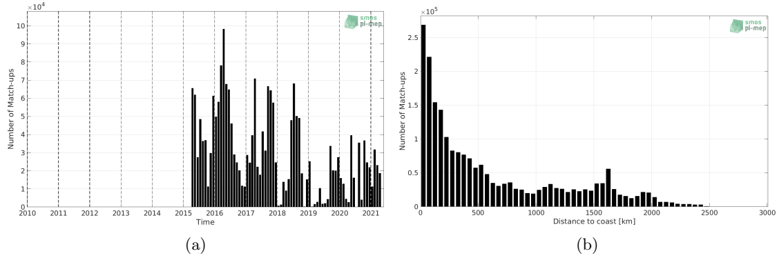
Figure 1: Number of match-ups between TSG (SAMOS) and SMAP SSS L3 v4 - 8-Day running (RSS) SSS as a function of time (a) and as function of the distance to coast (b) over the Tropical Pacific Ocean Pi-MEP region and for the full satellite product period.
