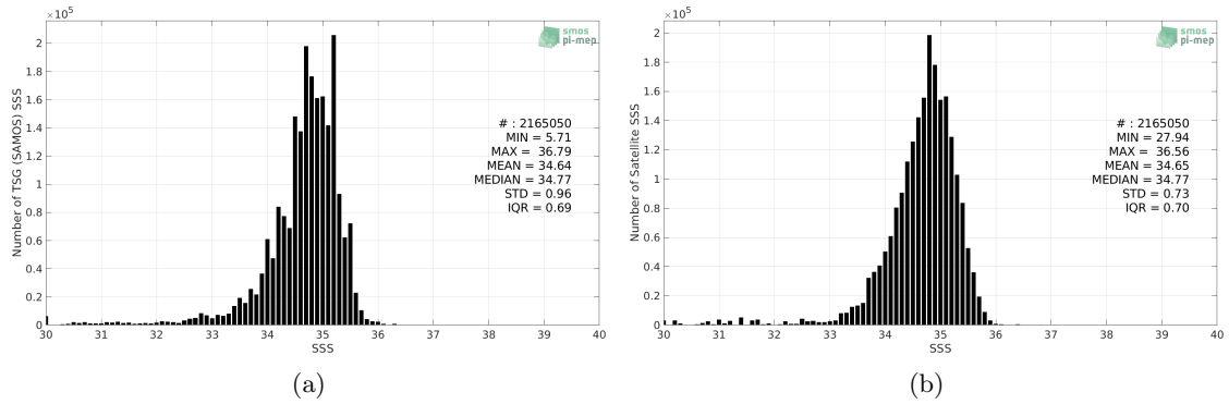
Figure 2: Histograms of SSS from TSG (SAMOS) (a) and SMAP SSS L3 v4 - 8-Day running (RSS) (b) considering all match-up pairs per bins of 0.1 over the Tropical Pacific Ocean Pi-MEP region and for the full satellite product period.
