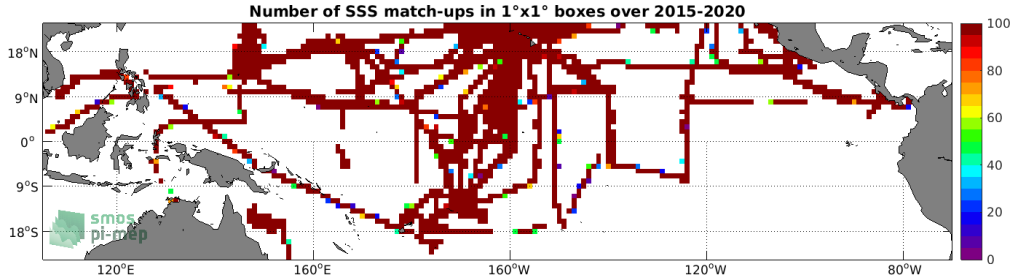
Figure 4: Number of SSS match-ups between TSG (SAMOS) SSS and the SMAP SSS L3 v4 - 8-Day running (RSS) SSS product for the Tropical Pacific Ocean Pi-MEP region over 1^\circ \times 1^\circ boxes and for the full satellite product period.
