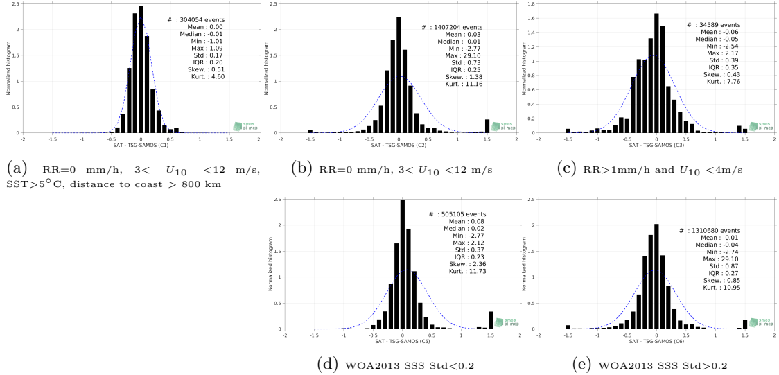
Figure 13: Normalized histogram of \Delta SSS (SMAP-L3-RSS-V4-8DAY-RUNNING - TSG-SAMOS) for 5 different subdatasets corresponding to: RR=0 mm/h, 3 < U_{10} < 12 m/s, SST >5^\circ\text{C} , distance to coast > 800 km (a), RR=0 mm/h, 3 < U_{10} < 12 m/s (b), RR >1 mm/h and U_{10} < 4 m/s (c), WOA2013 SSS Std <0.2 (d), WOA2013 SSS Std >0.2 (e).
