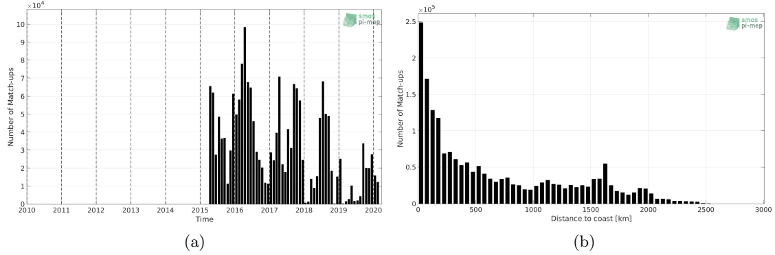
Figure 1: Number of match-ups between TSG-SAMOS and SMAP-L3-RSS-V4-8DAY-RUNNING SSS as a function of time (a) and as function of the distance to coast (b) over the Tropical Pacific Ocean Pi-MEP region and for the full satellite product period.
