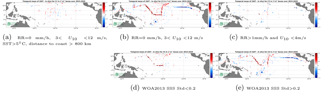
Figure 12: Temporal mean gridded over spatial boxes of size 1^\circ \times 1^\circ of \Delta SSS (SMAP-L3-RSS-V4-8DAY-RUNNING - TSG-SAMOS) for 5 different subdatasets corresponding to: RR=0 mm/h, 3 < U_{10} < 12 m/s, SST >5^\circ\text{C} , distance to coast > 800 km (a), RR=0 mm/h, 3 < U_{10} < 12 m/s (b), RR >1 mm/h and U_{10} < 4 m/s (c), WOA2013 SSS Std <0.2 (d), WOA2013 SSS Std >0.2 (e).
