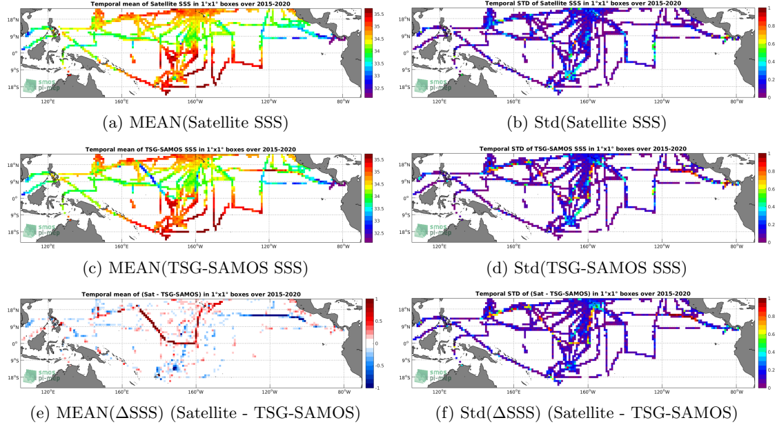
Figure 6: Temporal mean (left) and Std (right) of SSS from SMAP-L3-RSS-V4-8DAY-RUNNING (top), TSG-SAMOS (middle), and of \Delta SSS (Satellite - TSG-SAMOS). Only match-up pairs are used to generate these maps.
