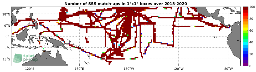
Figure 4: Number of SSS match-ups between TSG-SAMOS SSS and the SMAP-L3-RSS-V4-8DAY-RUNNING SSS product for the Tropical Pacific Ocean Pi-MEP region over 1^\circ \times 1^\circ boxes and for the full satellite product period.
