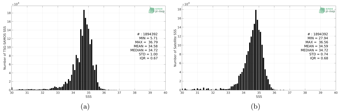
Figure 2: Histograms of SSS from TSG-SAMOS (a) and SMAP-L3-RSS-V4-8DAY-RUNNING (b) considering all match-up pairs per bins of 0.1 over the Tropical Pacific Ocean Pi-MEP region and for the full satellite product period.
