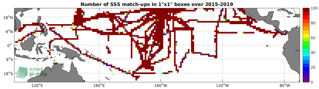
Figure 4: Number of SSS match-ups between TSG-SAMOS SSS and the SMAP-L3-RSS-V4-8DAY-RUNNING SSS product for the Tropical Pacific Ocean Pi-MEP region over 1^\circ \times 1^\circ boxes and for the full satellite product period.
