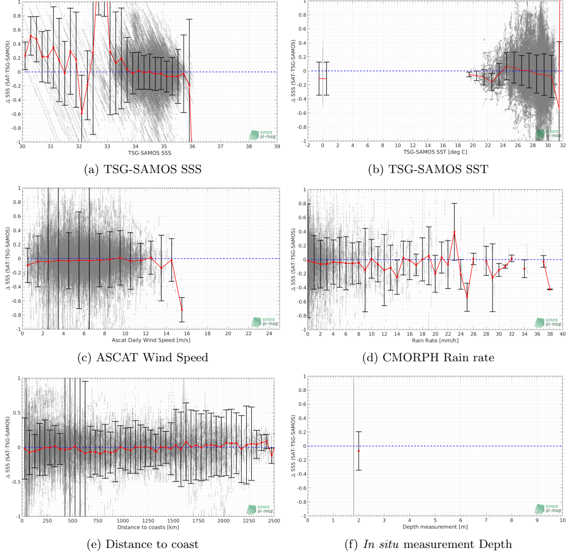
Figure 11: \Delta SSS (Satellite - TSG-SAMOS) sorted as function of TSG-SAMOS SSS values a), TSG-SAMOS SST b), ASCAT Wind speed c), CMORPH rain rate d), distance to coast (e) and in situ measurement depth (f). In all plots the median and Std of \Delta SSS for each bin is indicated by the red curves and black vertical thick bars ( \pm 1 Std)
