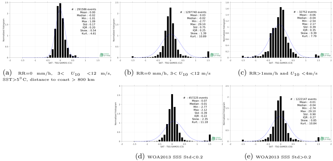
Figure 13: Normalized histogram of \Delta SSS (SMAP-L3-RSS-V4-8DAY-RUNNING - TSG-SAMOS) for 5 different subdatasets corresponding to: RR=0 mm/h, 3 < U_{10} < 12 m/s, SST > 5^\circ C , distance to coast > 800 km (a), RR=0 mm/h, 3 < U_{10} < 12 m/s (b), RR > 1 mm/h and U_{10} < 4 m/s (c), WOA2013 SSS Std < 0.2 (d), WOA2013 SSS Std > 0.2 (e).
