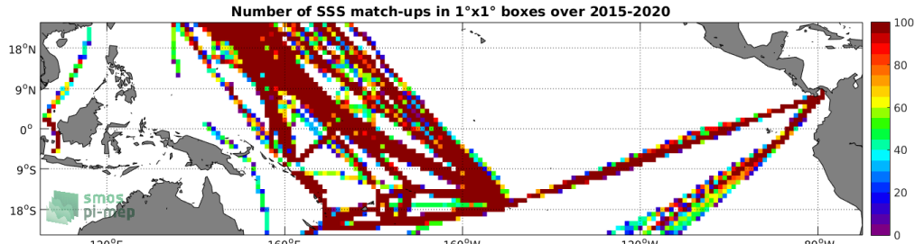
Figure 4: Number of SSS match-ups between TSG (LEGOS-DM) SSS and the SMAP SSS L3 v4 - 8-Day running (RSS) SSS product for the Tropical Pacific Ocean Pi-MEP region over 1^\circ \times 1^\circ boxes and for the full satellite product period.
