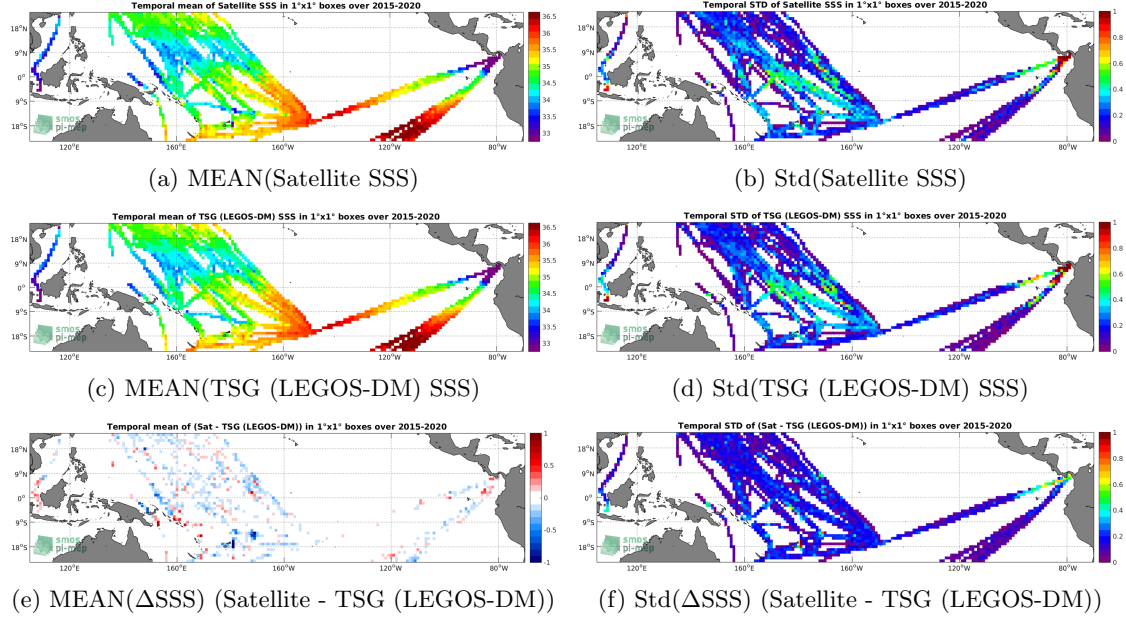
Figure 6: Temporal mean (left) and Std (right) of SSS from SMAP SSS L3 v4 - 8-Day running (RSS) (top), TSG (LEGOS-DM) (middle), and of \Delta SSS (Satellite - TSG (LEGOS-DM)). Only match-up pairs are used to generate these maps.
