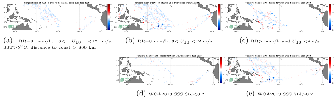
Figure 12: Temporal mean gridded over spatial boxes of size 1^\circ \times 1^\circ of \Delta SSS (SMAP SSS L3 v4 - 8-Day running (RSS) - TSG (LEGOS-DM)) for 5 different subdatasets corresponding to: RR=0 mm/h, 3 < U_{10} < 12 m/s, SST > 5^\circ C , distance to coast > 800 km (a), RR=0 mm/h, 3 < U_{10} < 12 m/s (b), RR > 1 mm/h and U_{10} < 4 m/s (c), WOA2013 SSS Std < 0.2 (d), WOA2013 SSS Std > 0.2 (e).
