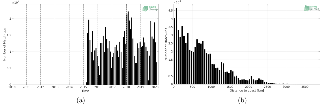
Figure 1: Number of match-ups between TSG (LEGOS-DM) and SMAP SSS L3 v4 - 8-Day running (RSS) SSS as a function of time (a) and as function of the distance to coast (b) over the Tropical Pacific Ocean Pi-MEP region and for the full satellite product period.
