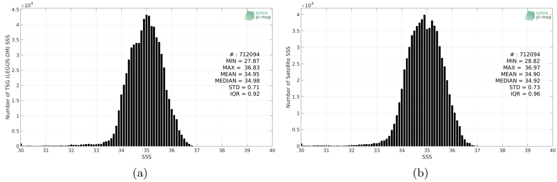
Figure 2: Histograms of SSS from TSG (LEGOS-DM) (a) and SMAP SSS L3 v4 - 8-Day running (RSS) (b) considering all match-up pairs per bins of 0.1 over the Tropical Pacific Ocean Pi-MEP region and for the full satellite product period.
