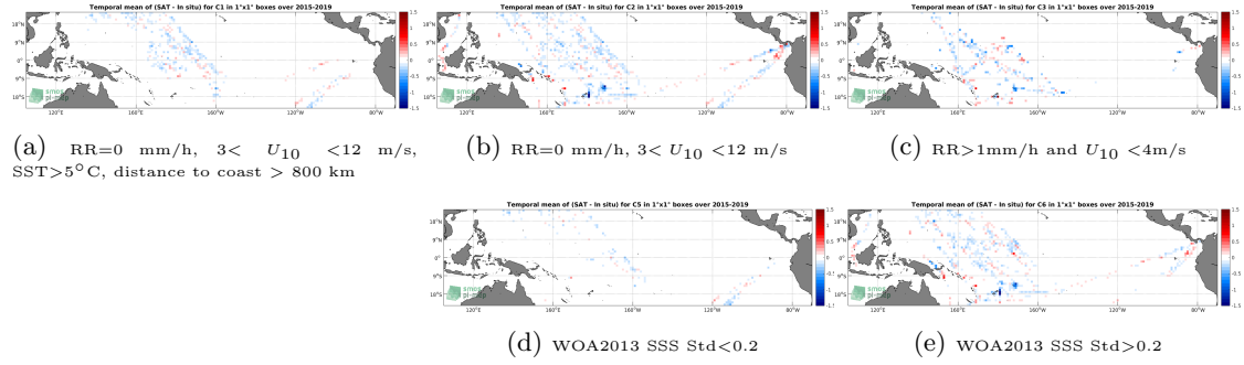
Figure 12: Temporal mean gridded over spatial boxes of size 1^\circ \times 1^\circ of \Delta SSS (SMAP-L3-RSS-V4-8DAY-RUNNING - TSG-LEGOS-DM) for 5 different subdatasets corresponding to: RR=0 mm/h, 3 < U_{10} < 12 m/s, SST > 5^\circ C , distance to coast > 800 km (a), RR=0 mm/h, 3 < U_{10} < 12 m/s (b), RR > 1 mm/h and U_{10} < 4 m/s (c), WOA2013 SSS Std < 0.2 (d), WOA2013 SSS Std > 0.2 (e).
