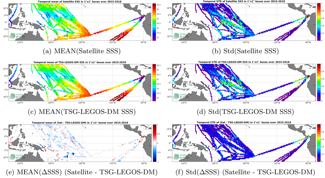
Figure 6: Temporal mean (left) and Std (right) of SSS from SMAP-L3-RSS-V4-8DAY-RUNNING (top), TSG-LEGOS-DM (middle), and of \Delta SSS (Satellite - TSG-LEGOS-DM). Only match-up pairs are used to generate these maps.
