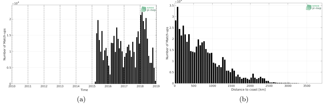
Figure 1: Number of match-ups between TSG-LEGOS-DM and SMAP-L3-RSS-V4-8DAY-RUNNING SSS as a function of time (a) and as function of the distance to coast (b) over the Tropical Pacific Ocean Pi-MEP region and for the full satellite product period.
