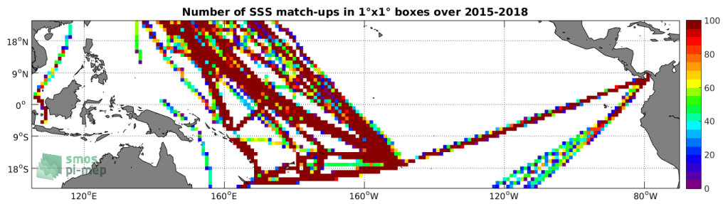
Figure 4: Number of SSS match-ups between TSG-LEGOS-DM SSS and the SMAP-L3-RSS-V4-8DAY-RUNNING SSS product for the Tropical Pacific Ocean Pi-MEP region over 1^\circ \times 1^\circ boxes and for the full satellite product period.
