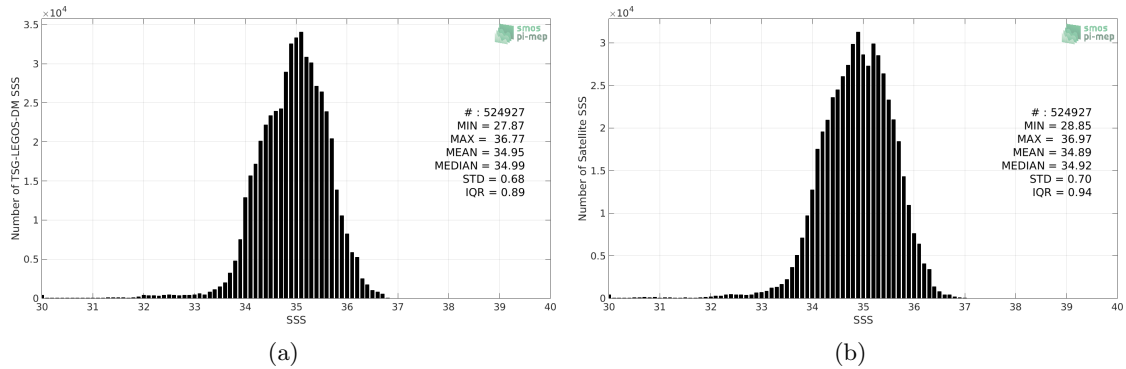
Figure 2: Histograms of SSS from TSG-LEGOS-DM (a) and SMAP-L3-RSS-V4-8DAY-RUNNING (b) considering all match-up pairs per bins of 0.1 over the Tropical Pacific Ocean Pi-MEP region and for the full satellite product period.
