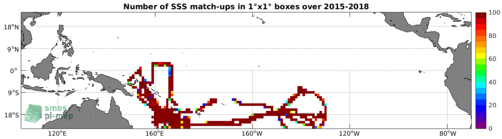
Figure 4: Number of SSS match-ups between TSG (GOSUD-Research-vessel) SSS and the SMAP SSS L3 v4 - 8-Day running (RSS) SSS product for the Tropical Pacific Ocean Pi-MEP region over 1^\circ \times 1^\circ boxes and for the full satellite product period.
