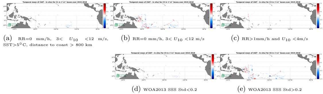
Figure 12: Temporal mean gridded over spatial boxes of size 1^\circ \times 1^\circ of \Delta SSS (SMAP SSS L3 v4 - 8-Day running (RSS) - TSG (GOSUD-Research-vessel)) for 5 different subdatasets corresponding to: RR=0 mm/h, 3 < U_{10} < 12 m/s, SST > 5^\circ\text{C} , distance to coast > 800 km (a), RR=0 mm/h, 3 < U_{10} < 12 m/s (b), RR > 1 mm/h and U_{10} < 4 m/s (c), WOA2013 SSS Std < 0.2 (d), WOA2013 SSS Std > 0.2 (e).
