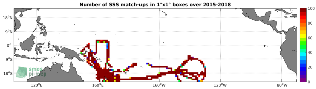
Figure 4: Number of SSS match-ups between TSG-GOSUD-Research-vessel SSS and the SMAP-L3-RSS-V4-8DAY-RUNNING SSS product for the Tropical Pacific Ocean Pi-MEP region over 1^\circ \times 1^\circ boxes and for the full satellite product period.
