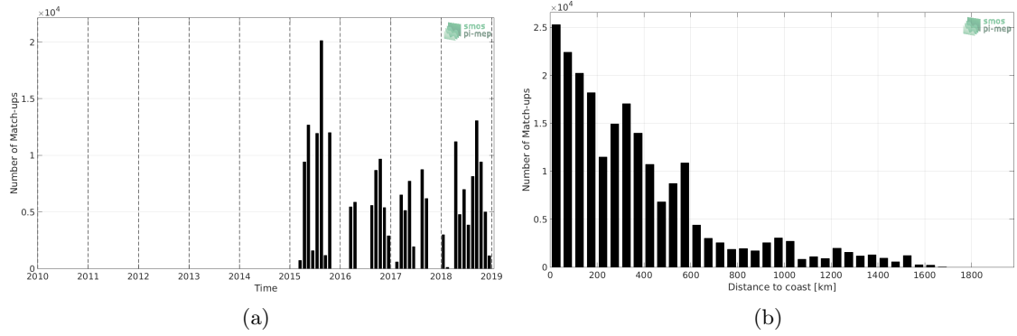
Figure 1: Number of match-ups between TSG-GOSUD-Research-vessel and SMAP-L3-RSS-V4-8DAY-RUNNING SSS as a function of time (a) and as function of the distance to coast (b) over the Tropical Pacific Ocean Pi-MEP region and for the full satellite product period.
