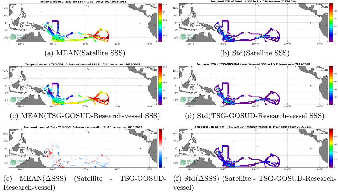
Figure 6: Temporal mean (left) and Std (right) of SSS from SMAP-L3-RSS-V4-8DAY-RUNNING (top), TSG-GOSUD-Research-vessel (middle), and of \Delta SSS (Satellite - TSG-GOSUD-Research-vessel). Only match-up pairs are used to generate these maps.
