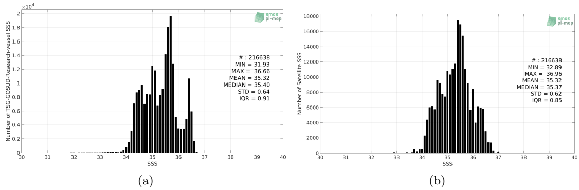
Figure 2: Histograms of SSS from TSG-GOSUD-Research-vessel (a) and SMAP-L3-RSS-V4-8DAY-RUNNING (b) considering all match-up pairs per bins of 0.1 over the Tropical Pacific Ocean Pi-MEP region and for the full satellite product period.
