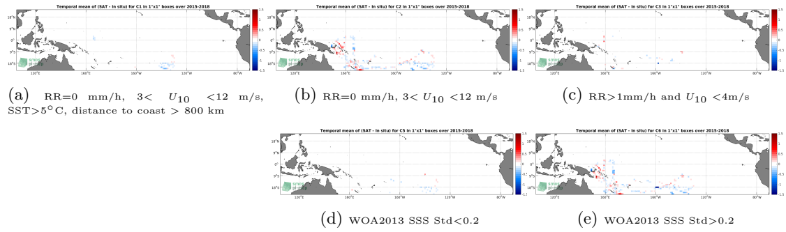
Figure 12: Temporal mean gridded over spatial boxes of size 1^\circ \times 1^\circ of \Delta SSS (SMAP-L3-RSS-V4-8DAY-RUNNING - TSG-GOSUD-Research-vessel) for 5 different subdatasets corresponding to: RR=0 mm/h, 3 < U_{10} < 12 m/s, SST > 5^\circ C , distance to coast > 800 km (a), RR=0 mm/h, 3 < U_{10} < 12 m/s (b), RR > 1 mm/h and U_{10} < 4 m/s (c), WOA2013 SSS Std < 0.2 (d), WOA2013 SSS Std > 0.2 (e).
