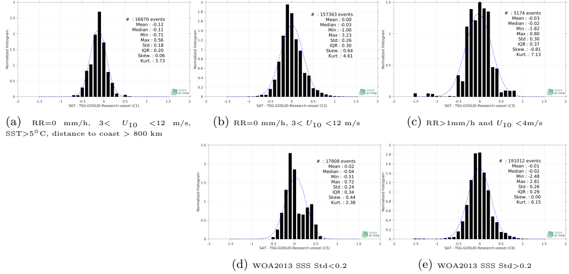
Figure 13: Normalized histogram of \Delta SSS (SMAP-L3-RSS-V4-8DAY-RUNNING - TSG-GOSUD-Research-vessel) for 5 different subdatasets corresponding to: RR=0 mm/h, 3 < U_{10} < 12 m/s, SST>5°C, distance to coast > 800 km (a), RR=0 mm/h, 3 < U_{10} < 12 m/s (b), RR>1mm/h and U_{10} < 4 m/s (c), WOA2013 SSS Std<0.2 (d), WOA2013 SSS Std>0.2 (e).
