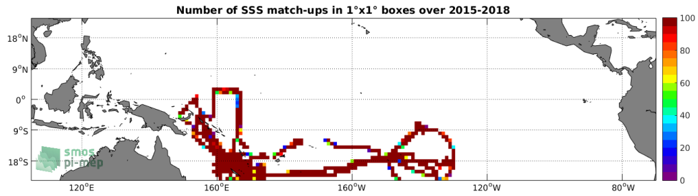
Figure 4: Number of SSS match-ups between TSG-GOSUD-Research-vessel SSS and the SMAP-L3-RSS-V4-8DAY-RUNNING SSS product for the Tropical Pacific Ocean Pi-MEP region over 1°x1° boxes and for the full satellite product period.
