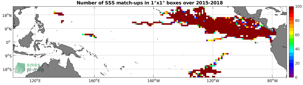
Figure 3: Number of SSS match-ups between Surface drifters SSS and the SMAP SSS L3 v4 - 8-Day running (RSS) SSS product for the Tropical Pacific Ocean Pi-MEP region over 1^\circ \times 1^\circ boxes and for the full satellite product period.
